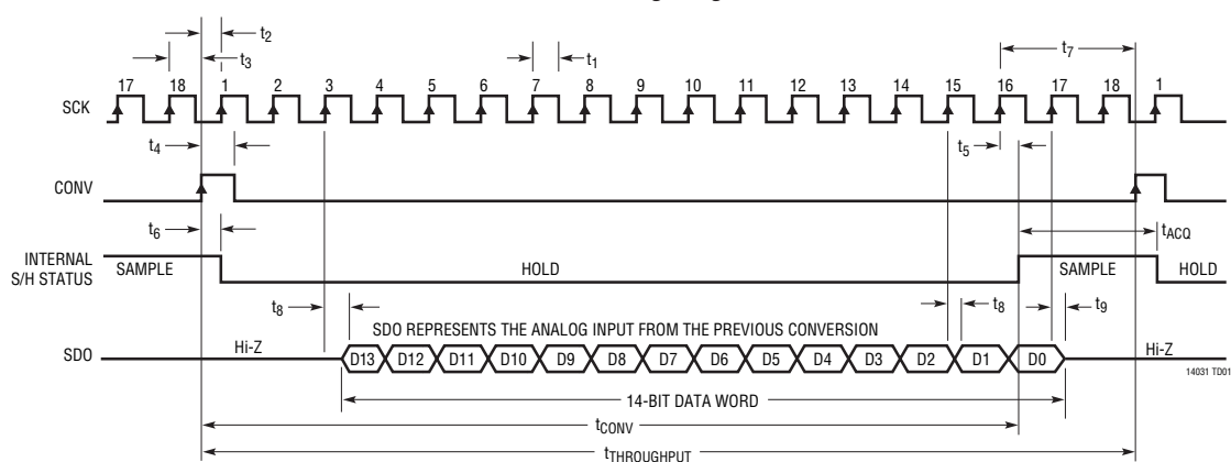
LTC1403A Timing Diagram
