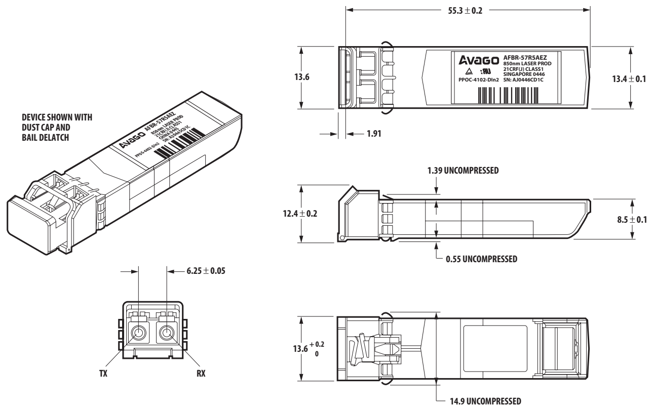
Figure 5. Module drawing.
