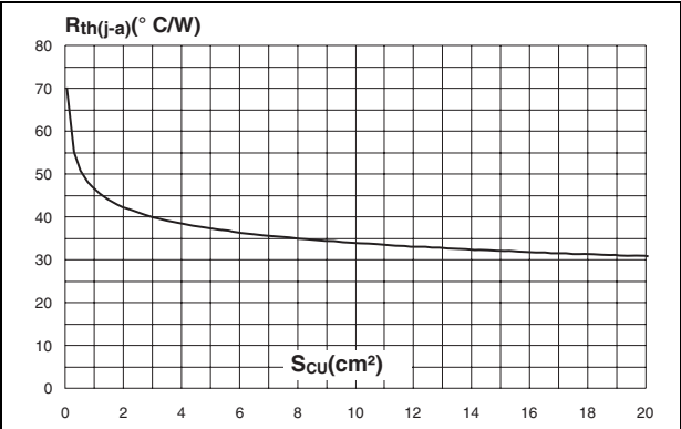
Figure 10. Thermal resistance junction to ambient versus copper surface under each tab (Epoxy printed circuit board FR4, e_{\text{CU}} = 35\text{ }\mu\text{m} ) for D 2 PAK
