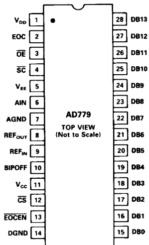
DIP Package
