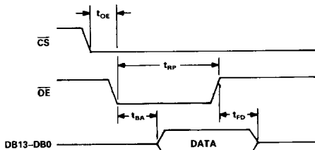
Figure 2. Output Timing
