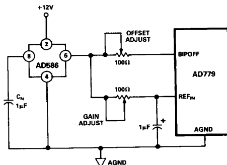
Figure 7. Bipolar Input with Gain and Offset Trims
