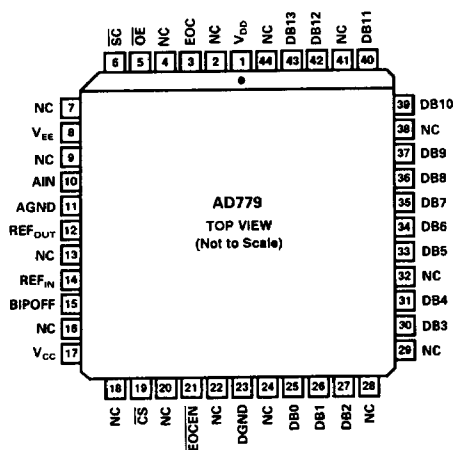
JLCC Package
