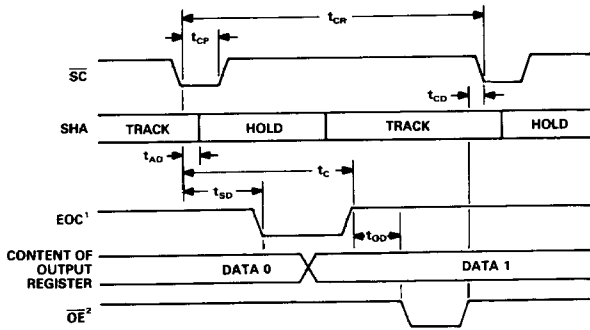
Figure 1. Conversion Timing
