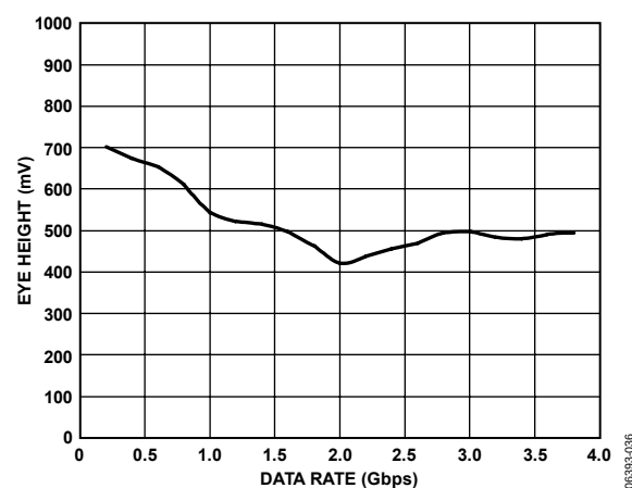
Figure 30. Eye Height vs. Data Rate
