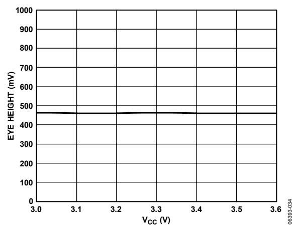
Figure 29. Eye Height vs. Core Supply Voltage
