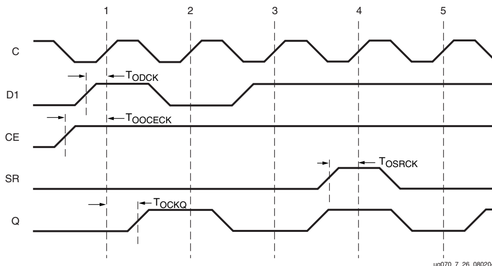
Figure 7-26: OLOGIC Output Register Timing Characteristics
