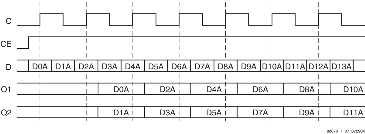
Figure 7-7: Input DDR Timing in SAME_EDGE_PIPELINED Mode
