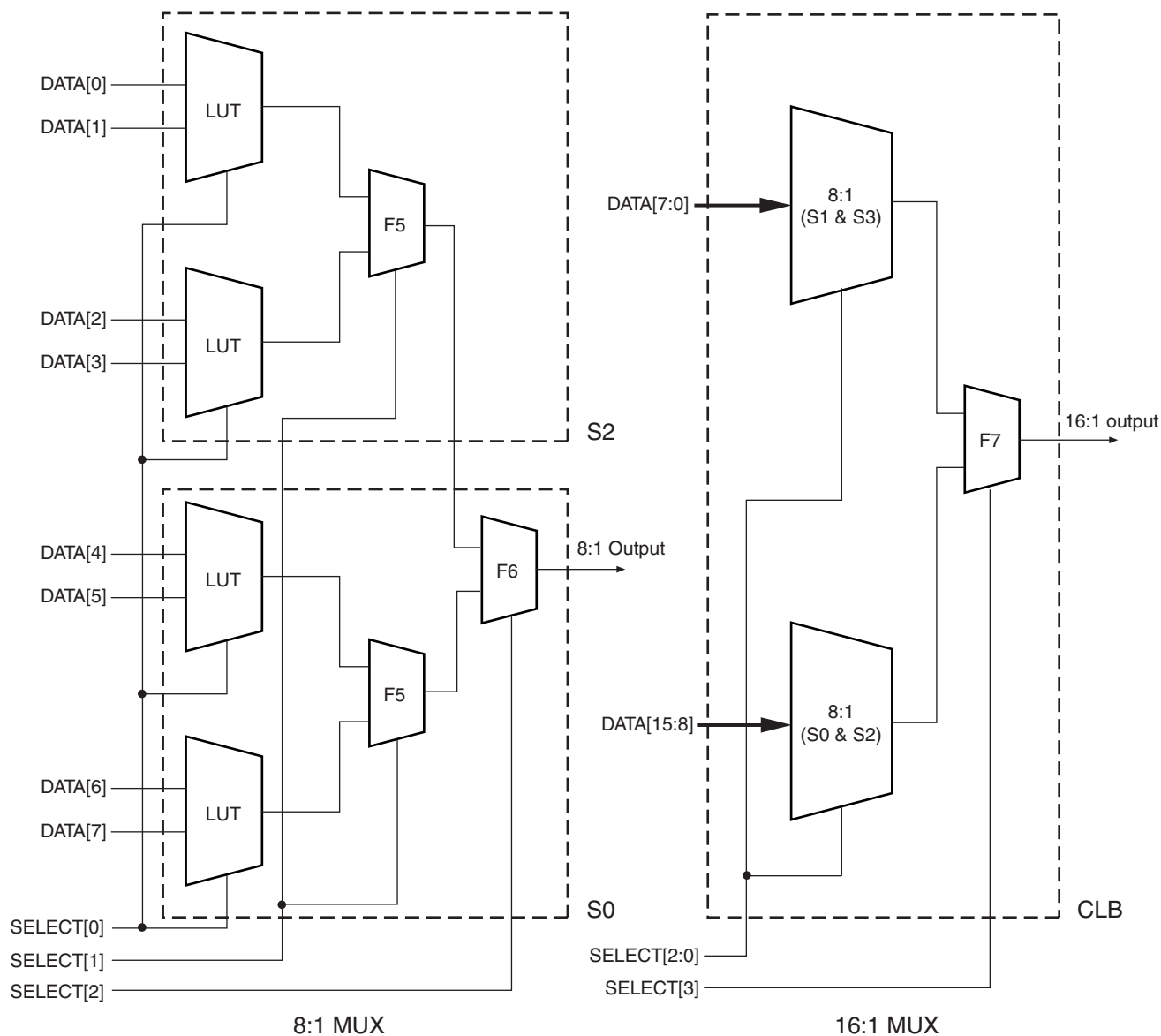
Figure 5-18: 8:1 and 16:1 Multiplexers
