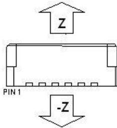
Figure 1. Accelerometer measuring directions.
