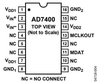
Figure 5. Pin Configuration
