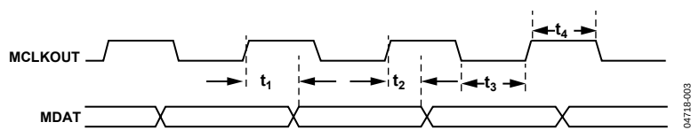
Figure 3. Data Timing
