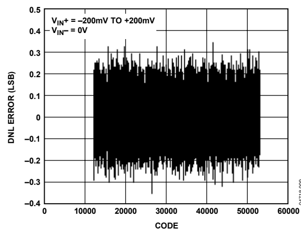
Figure 10. Typical DNL, \pm 200 mV Range (Using \text{Sinc}^3 Filter, 256 Decimation Rate)
