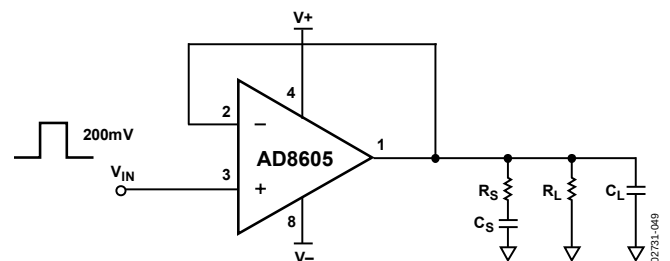
Figure 48. Snubber Network Configuration
