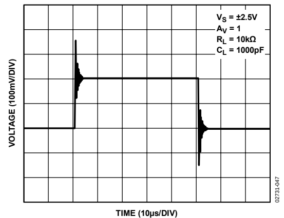
Figure 47. AD8606 Capacitive Load Drive Without Snubber
