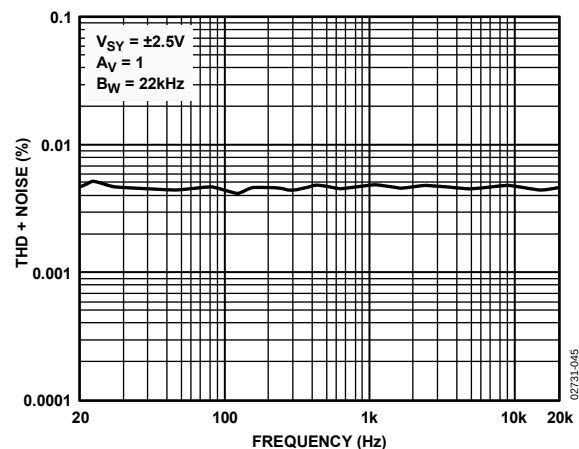
Figure 45. THD + Noise vs. Frequency
