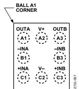
Figure 2. 8-Ball WLCSP (CB Suffix)
