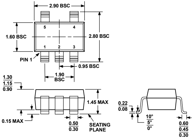
COMPLIANT TO JEDEC STANDARDS MO-178-AA Figure 58. 5-Lead Small Outline Transistor Package [SOT-23] (RJ-5) Dimensions shown in millimeters
