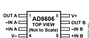
Figure 5. 8-Lead MSOP (RM Suffix) 8-Lead SOIC_N (R Suffix)
