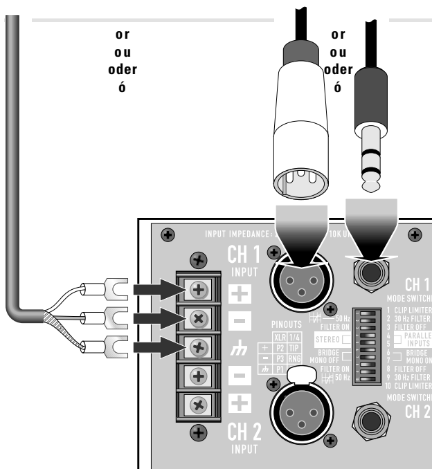
XLR unbalanced • XLR asymétrique • unsymmetrische XLR • XLR no balanceado
