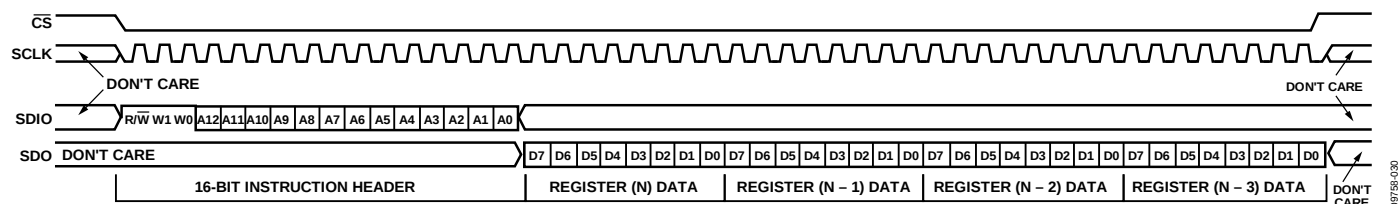
Figure 47. Serial Control Port Read—MSB First, 16-Bit Instruction, Four Bytes of Data
