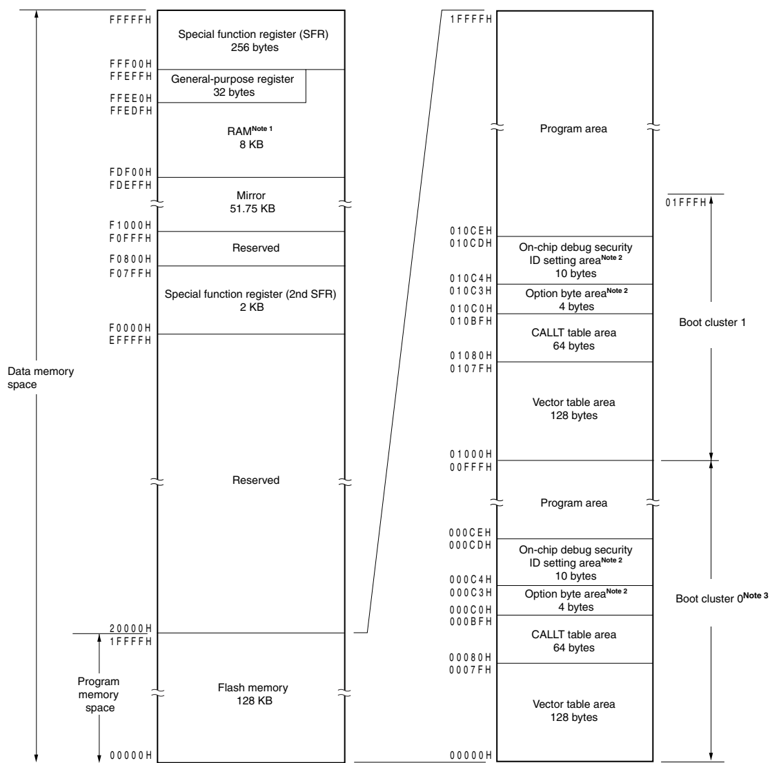
Figure 3-3. Memory Map ( \mu PD78F1154, 78F1154A)
