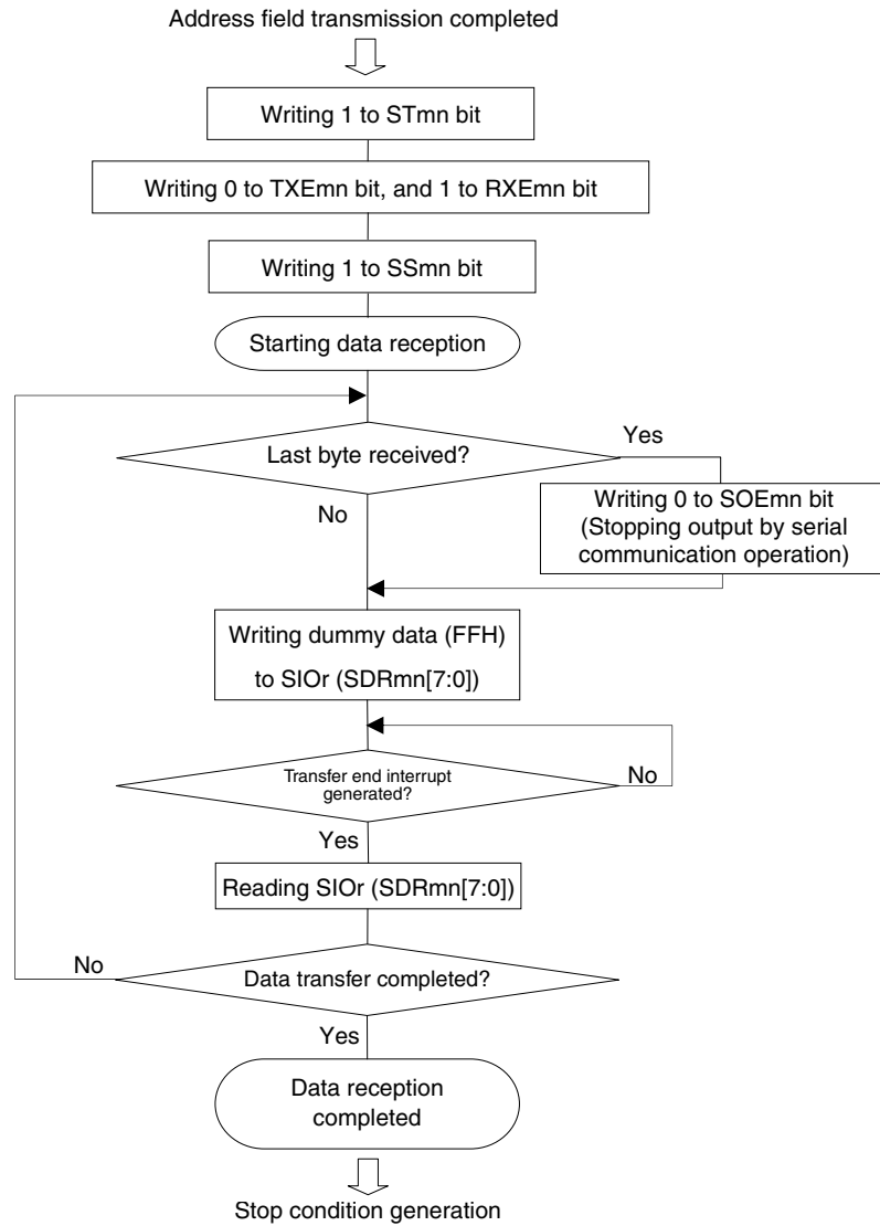
Figure 12-102. Flowchart of Data Reception
