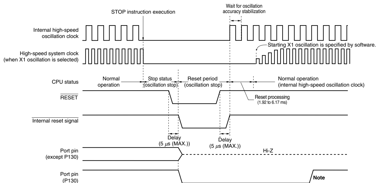
Figure 19-4. Timing of Reset in STOP Mode by RESET Input
