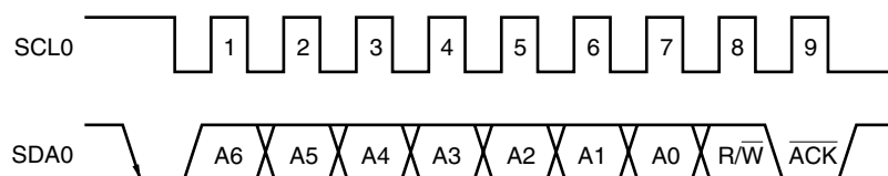
Figure 13-17. \overline{\text{ACK}}
