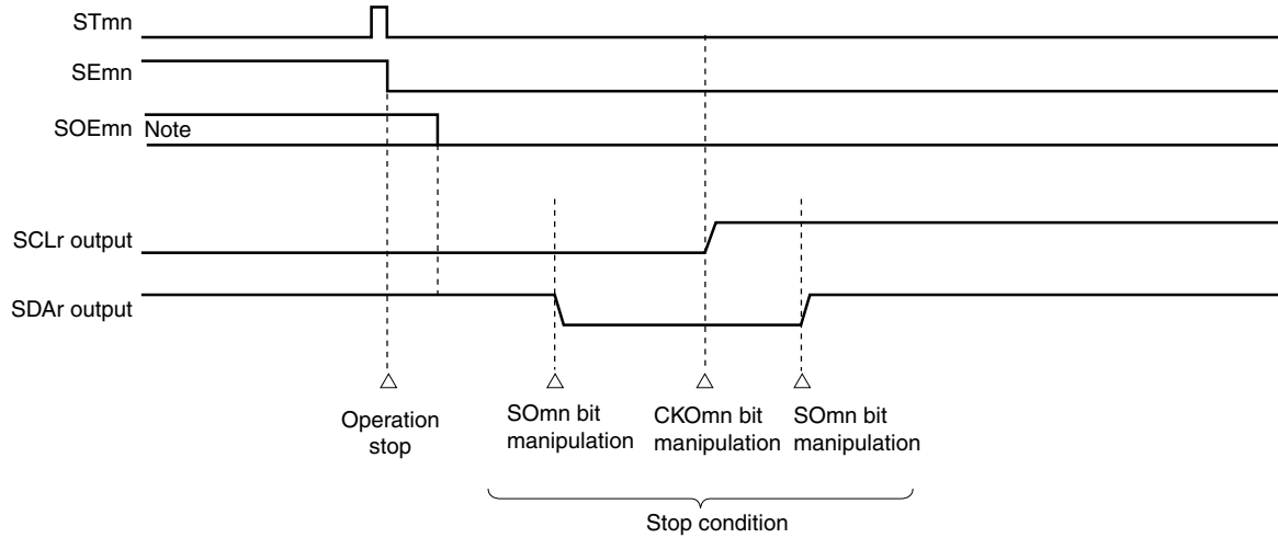
Figure 12-103. Timing Chart of Stop Condition Generation
