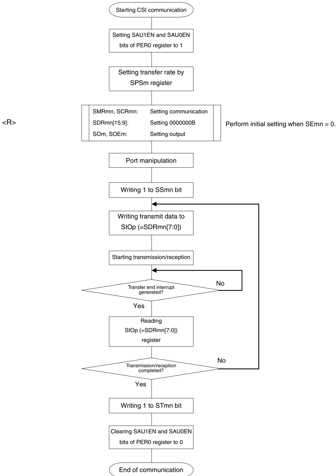
Figure 12-67. Flowchart of Slave Transmission/Reception (in Single- Transmission/Reception Mode)
