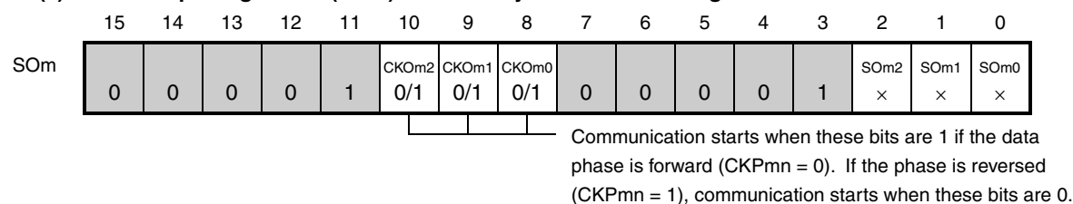
Figure 12-32. Example of Contents of Registers for Master Reception of 3-Wire Serial I/O (CSI00, CSI01, CSI10, CSI20)
