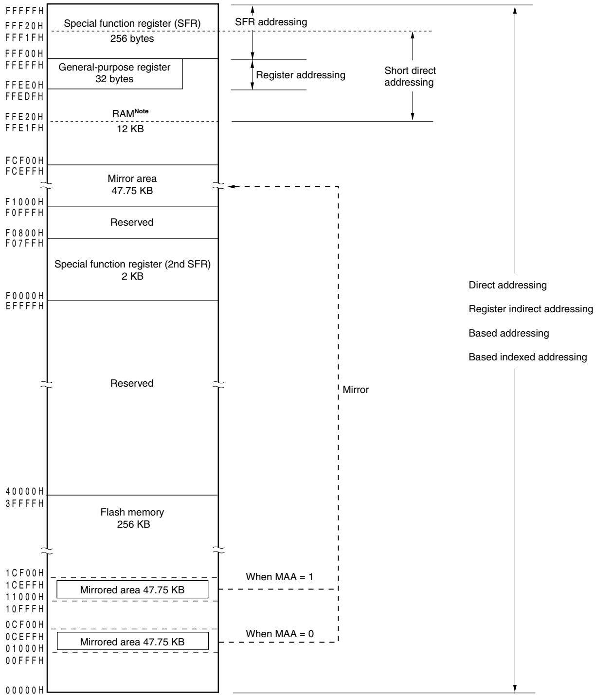
Figure 3-11. Correspondence Between Data Memory and Addressing ( \mu PD78F1156, 78F1156A)
