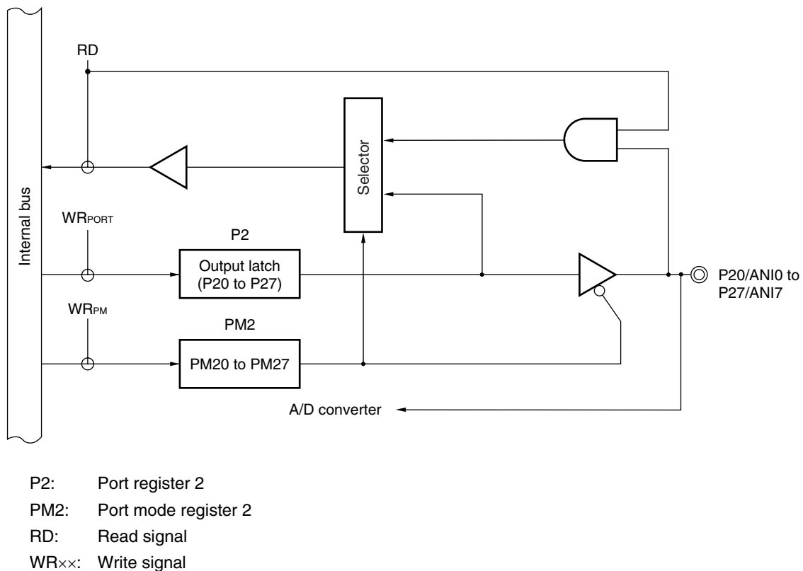
Figure 4-12. Block Diagram of P20 to P27
