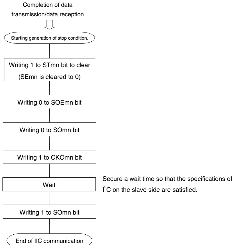
Figure 12-104. Flowchart of Stop Condition Generation
