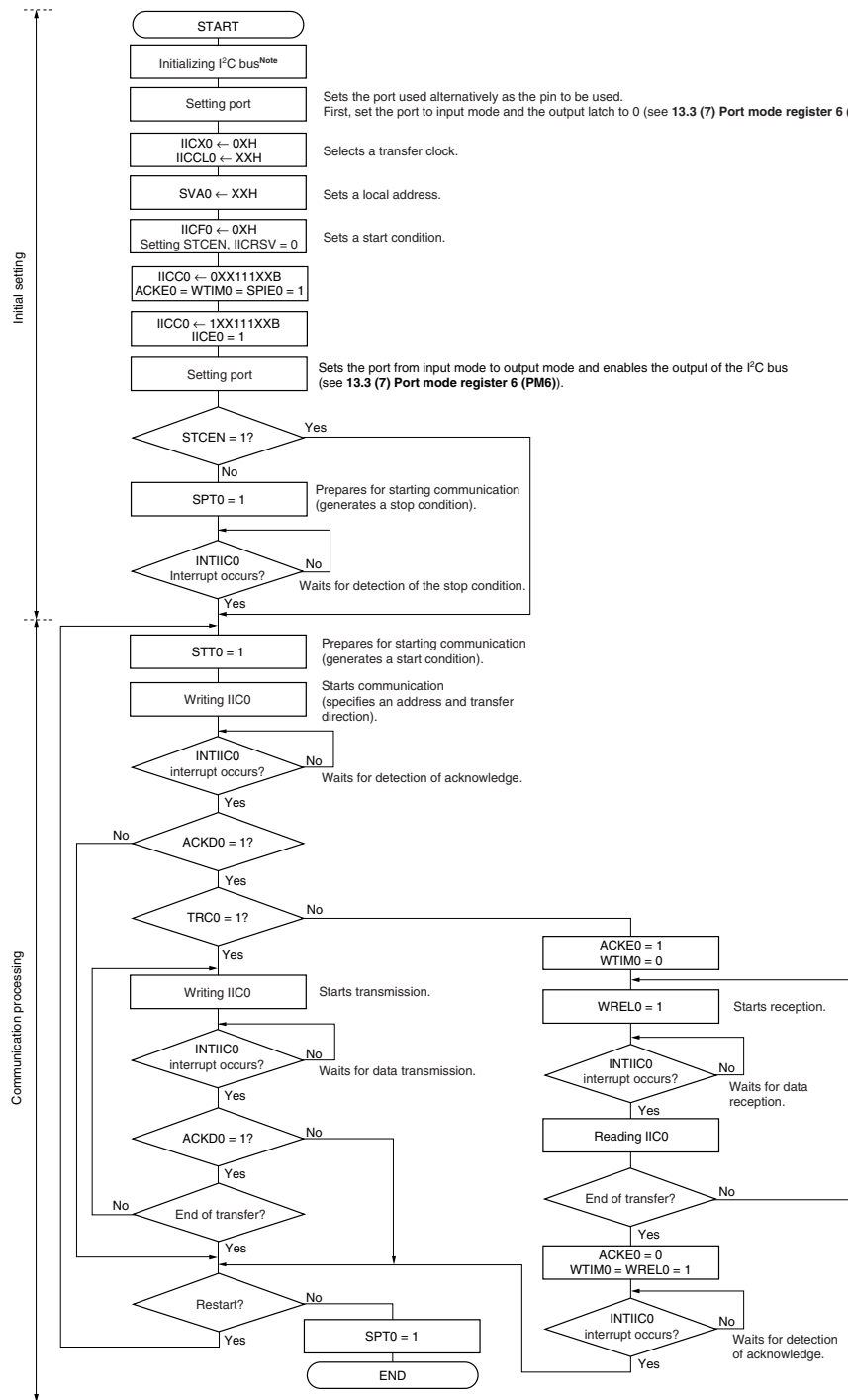
Figure 13-24. Master Operation in Single-Master System
