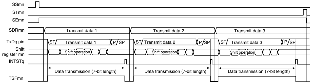
Figure 12-75. Timing Chart of UART Transmission (in Single-Transmission Mode)
