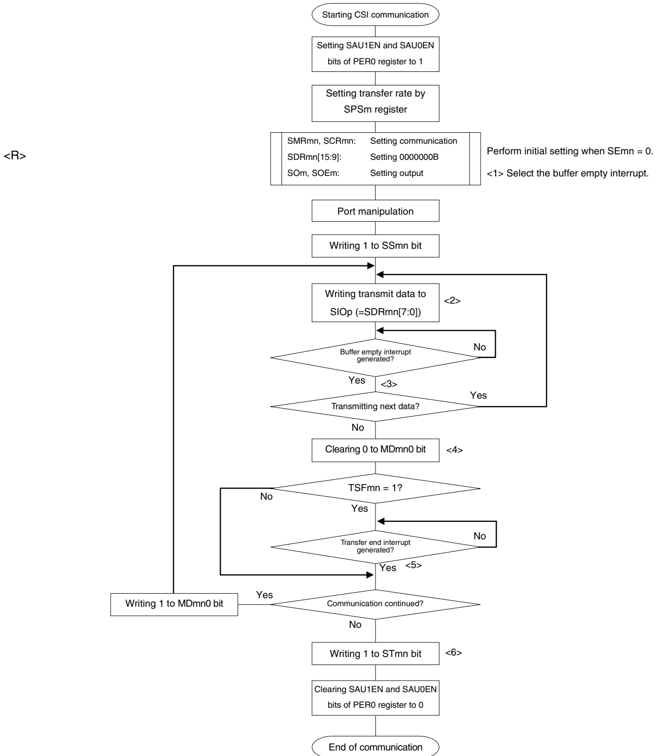
Figure 12-55. Flowchart of Slave Transmission (in Continuous Transmission Mode)
