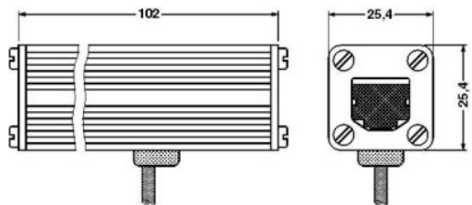
Dimensioned drawing
