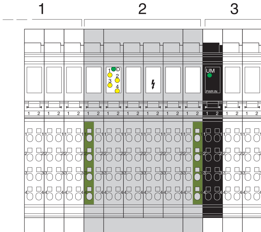
Connection diagram
