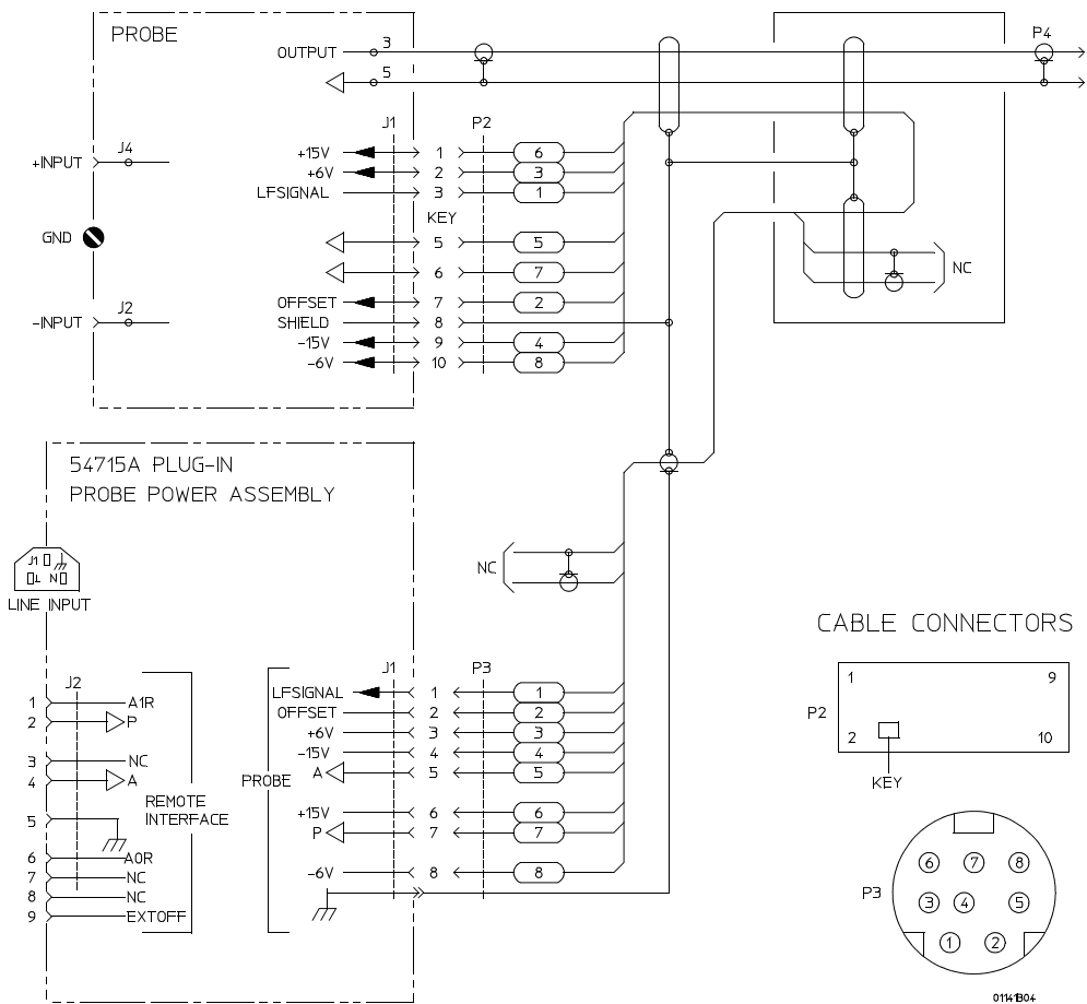
Cabling Diagram
