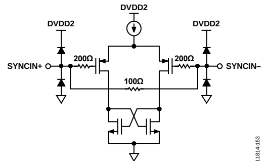
Figure 52. Equivalent SYNCIN± Input
