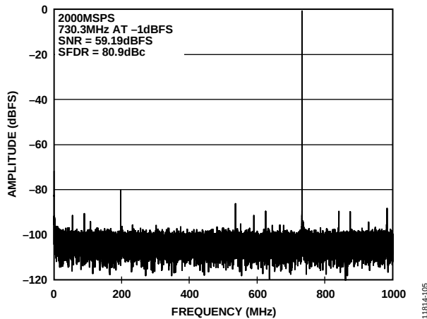
Figure 13. FFT Plot at 2.0 GSPS, f_{IN} = 730.3 MHz at AIN (SFDR = 80.9 dBc, SNR = 59.2 dBFS)
