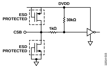
Figure 49. Equivalent CSB/PWDN Input Circuit
