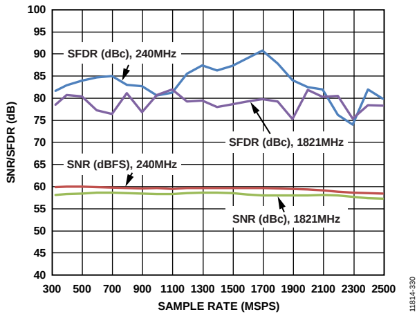
Figure 30. SNR/SFDR vs. Sample Rate
