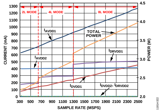
Figure 22. Current and Power vs. Sample Rate: 2 Lane, 4 Lane, and 8 Lane Output Modes
