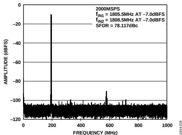
Figure 37. Two Tone FFT Plot at 2.0 GSps, f_{IN1} = 1805.5 MHz and f_{IN2} = 1808.5 MHz at AIN, -7 dBFS (SFDR = 78.1 dBc)
