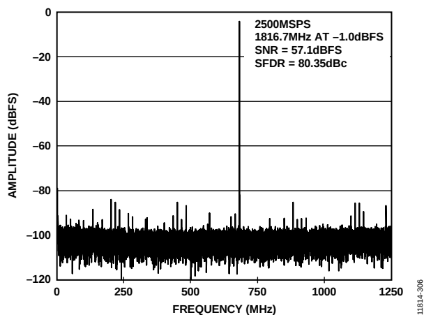
Figure 6. FFT Plot at 2.5 GSPS, f_{IN} = 1816.7 MHz at AIN (SFDR = 80.4 dBc, SNR = 57.1 dBFS)
