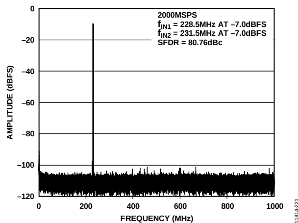
Figure 39. Two Tone FFT Plot at 2.0 GSps, f_{IN1} = 228.5 MHz and f_{IN2} = 231.5 MHz at AIN, -7 dBFS (SFDR = 81 dBc)
