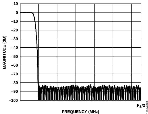
Figure 63. Magnitude Response of the Decimate-by-8 Polyphase Fuse Filter
