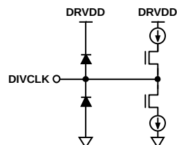
Figure 50. Equivalent DIVCLK Output Circuit (DRVDD)
