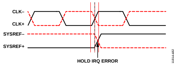
Figure 77. SYSREF± Edge Falls Within the Actual Hold Time Window and Triggers an IRQ Error
