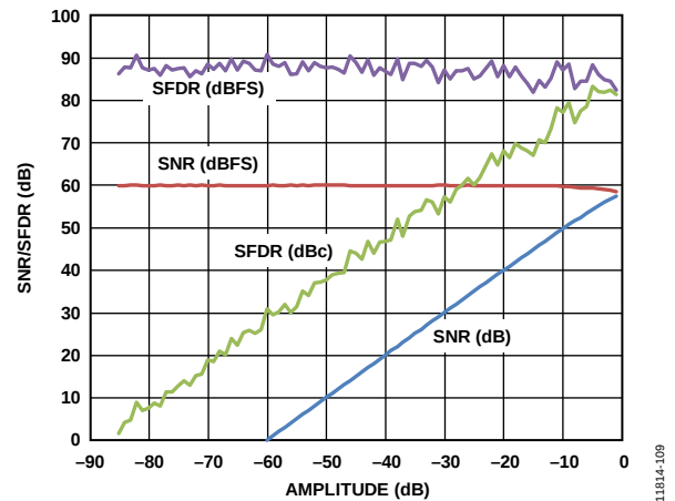
Figure 16. SNR/SFDR vs. Analog Input Amplitude at 2 GSPS, f_{IN} = 1811.3 MHz at AIN
