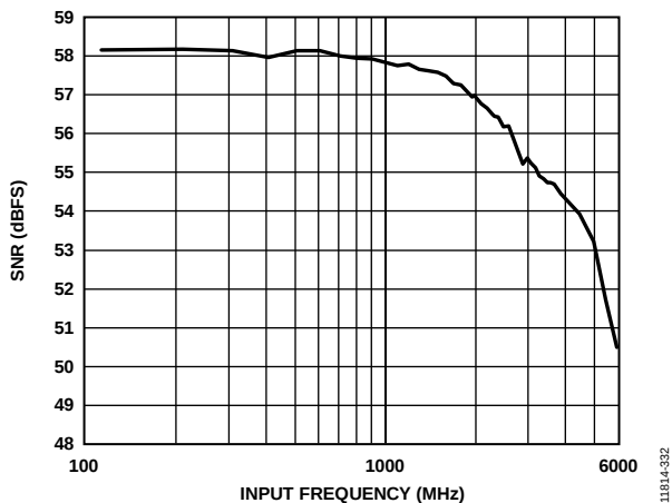
Figure 32. SNRFS vs. AIN Frequency at 2.5 GSPS (Input Network in Figure 60 Used &lt;2 GHz, Input Network in Figure 59 Used &gt;2 GHz)
