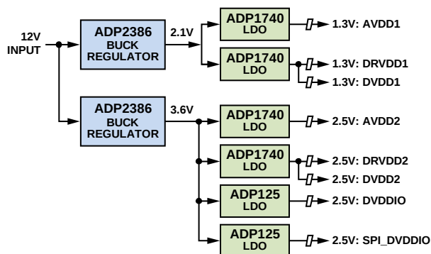
Figure 86. Power Supply Recommendation
