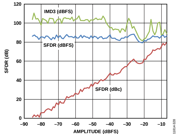
Figure 28. Two Tone SFDR and IMD3 vs. Analog Input Amplitude at 2.5 GSPS at 230 MHz AIN
