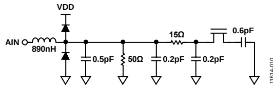
Figure 45. Equivalent Analog Input Circuit
