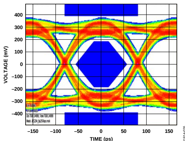
Figure 71. Recovered Data Eye of JESD204B Lane at 6.25 Gbps
