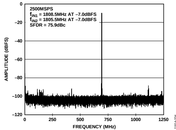
Figure 34. Two Tone FFT Plot at 2.5 GSPS, f_{IN1} = 1808.5 MHz and f_{IN2} = 1805.5 MHz at AIN, -7 dBFS (SFDR = 76 dBc)
