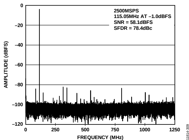
Figure 9. FFT Plot at 2.5 GSPS, f_{IN} = 115 MHz at AIN (SFDR = 78.4 dBc, SNR = 58.1 dBFS)
