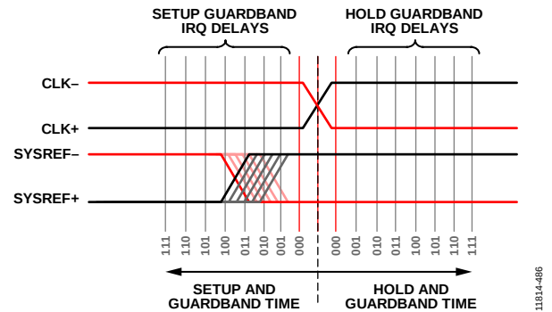
Figure 81. \text{SYSREF}\pm Edge Changes Phase Relative to the Encode Clock, Which can be Detected When the Edge Crosses Through the Guardband Setup Time
