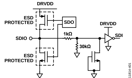
Figure 53. Equivalent SDIO Circuit
