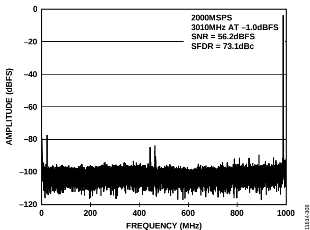
Figure 8. FFT Plot at 2.0 GSPS, f_{IN} = 3010 MHz at AIN (SFDR = 73 dBc, SNR = 56 dBFS) (Input Network in Figure 60 Used)
