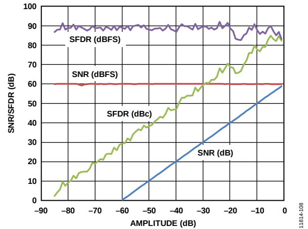
Figure 15. SNR/SFDR vs. Analog Input Amplitude at 2 GSPS, f_{IN} = 241.1 MHz at AIN
