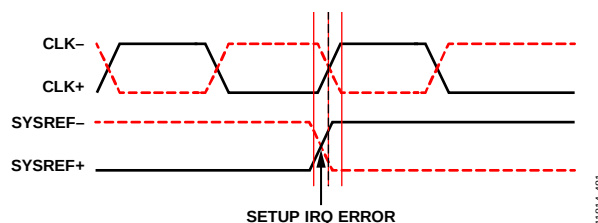
Figure 76. SYSREF± Edge Falls Within the Actual Setup Time Window and Triggers an IRQ Error
