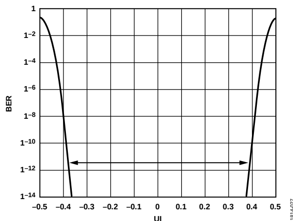
Figure 72. Bathtub Plot of JESD204B Output at 6.25 Gbps
