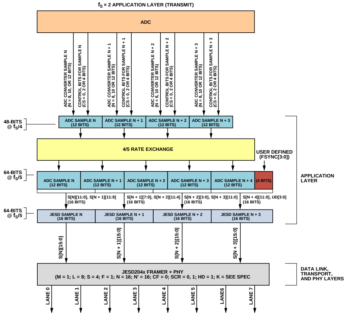
Figure 84. f_s \times 2 Mode Application Layer (Transmit)
