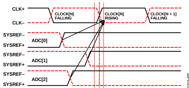
Figure 83. Changing the Latching Edge to Rising for All Three ADCs, SYSREF± Can Now be Aligned to CLK±[N]
