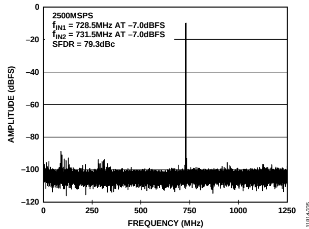
Figure 35. Two Tone FFT Plot at 2.5 GSPS, f_{IN1} = 728.5 MHz and f_{IN2} = 731.5 MHz at AIN, -7 dBFS (SFDR = 79 dBc)
