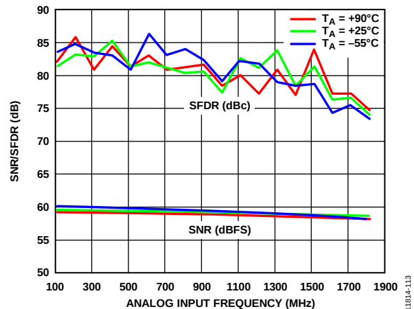
Figure 25. SNR/SFDR vs. Analog Input Frequency at Different Temperatures at 2.0 GSPS
