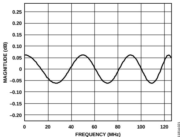
Figure 64. Magnitude Ripple in the High Bandwidth Pass Band
