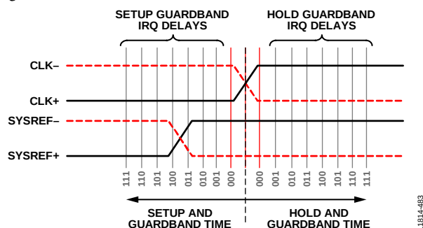
Figure 78. SYSREF± Edge Falls Within the Guardbanded Setup Time Window and Triggers an IRQ Error
