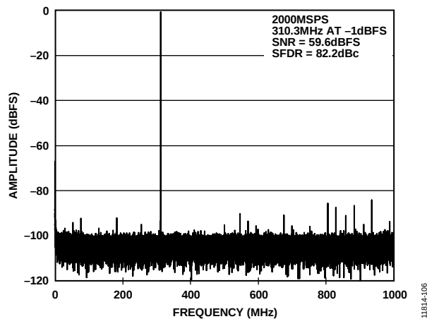
Figure 14. FFT Plot at 2.0 GSPS, f_{IN} = 310.3 MHz at AIN (SFDR = 82.2 dBc, SNR = 59.6 dBFS)
