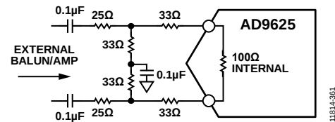
Figure 60. Input Network Example for Passive Balun and <2 GHz ADC Bandwidth
