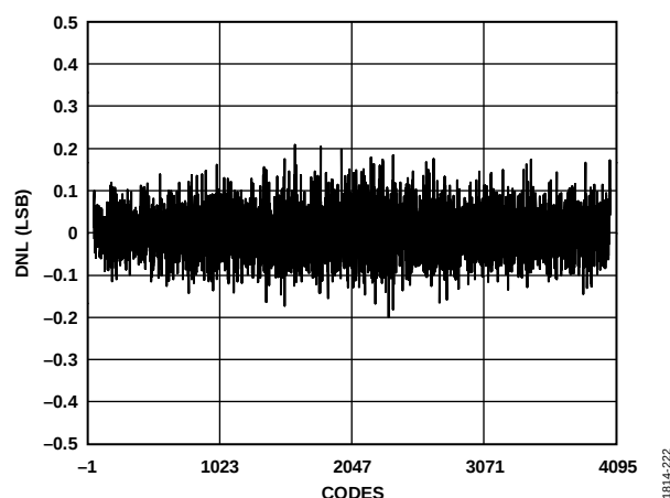
Figure 40. Differential Nonlinearity (DNL), \pm 0.2 LSB at 2.0 GSps
