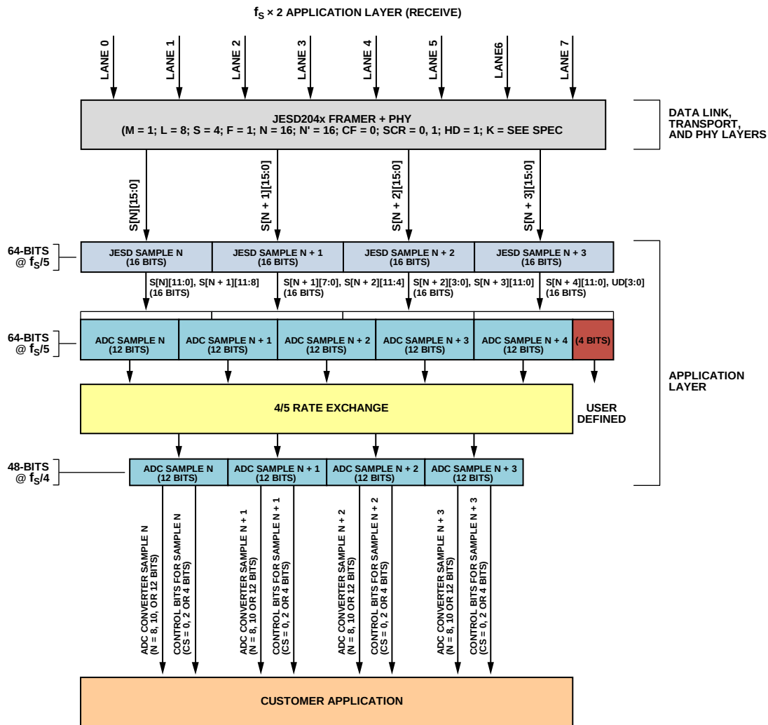
Figure 85. f_S \times 2 Application Layer (Receive)
