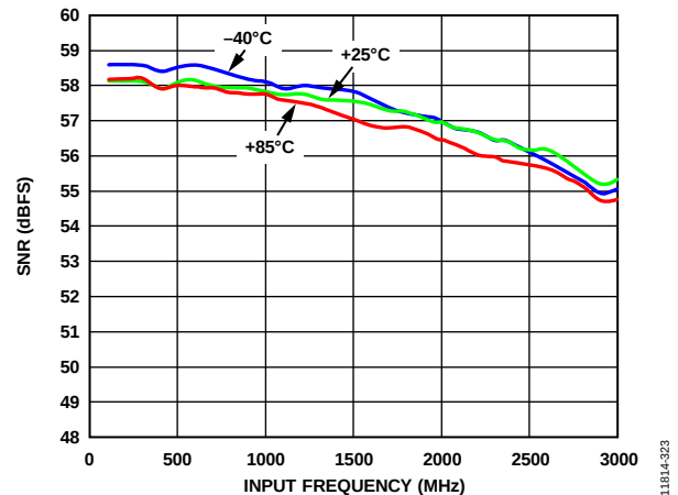
Figure 23. SNR at 2.5GSPS vs. Temperature (Input Network in Figure 60 Used <2 GHz, Input Network in Figure 59 Used >2 GHz)
