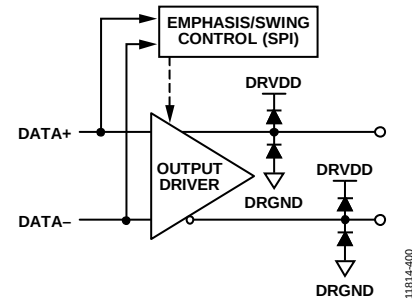
Figure 51. Digital Outputs
