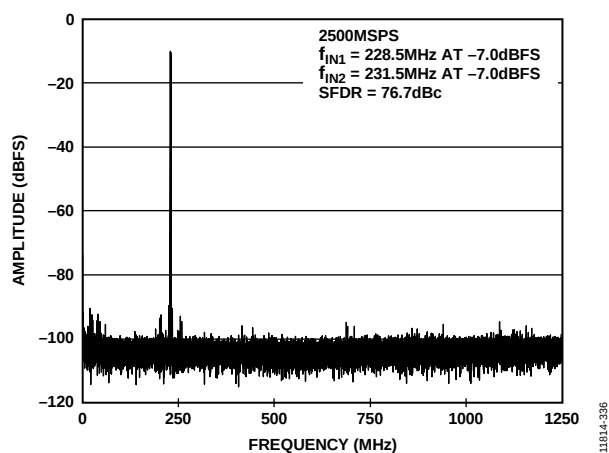
Figure 36. Two Tone FFT Plot at 2.5 GSps, f_{IN1} = 228.5 MHz and f_{IN2} = 231.5 MHz at AIN, -7 dBFS (SFDR = 76 dBc)
