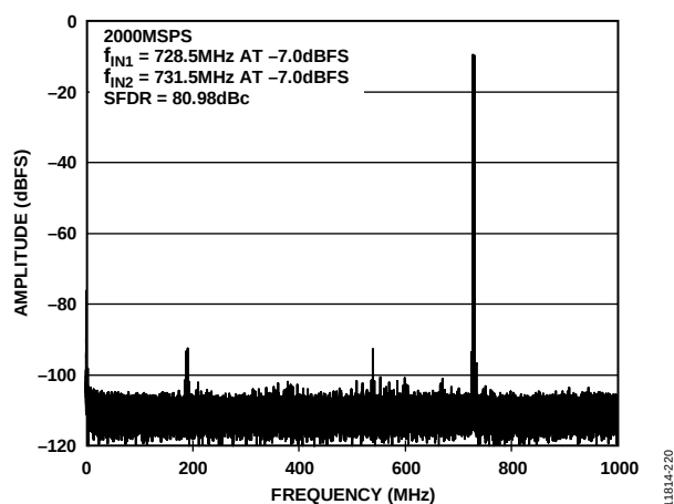
Figure 38. Two Tone FFT Plot at 2.0 GSps, f_{IN1} = 728.5 MHz and f_{IN2} = 731.5 MHz at AIN, -7 dBFS (SFDR = 81 dBc)
