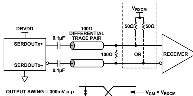
Figure 69. AC-Coupled Digital Output Termination Example
