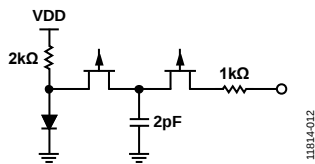
Figure 47. Equivalent VMON Temperature Sensor Circuit (DVDDD)
