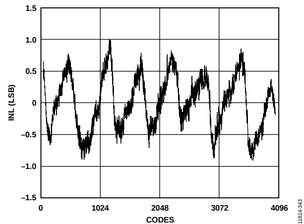
Figure 43. Integral Nonlinearity (INL), ±1.0 LSB at 2.5 GSPS
