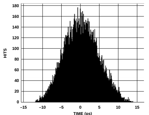
Figure 73. Time Interval Histogram Error of JESD204B Output at 6.25 Gbps
