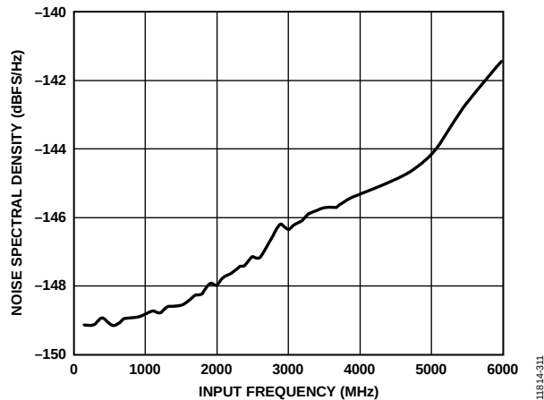
Figure 11. NSD vs. AIN at 2.5GSPS (Input Network in Figure 60 Used <2 GHz, Input Network in Figure 59 Used >2 GHz)
