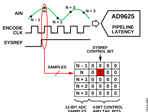
Figure 75. A SYSREF± Control Bit Can Be Used to Mark the Same Analog Sample that is Coincident with a Sampled SYSREF± Edge by CLK±
