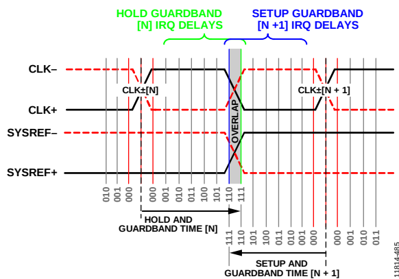
Figure 80. \text{SYSREF}\pm Edge Falls Within Both the Latest Hold Time Guardbanded of \text{CLK}\pm[N] and the Earliest Setup Time Guardband of \text{CLK}\pm[N+1] and Triggers an IRQ Error
