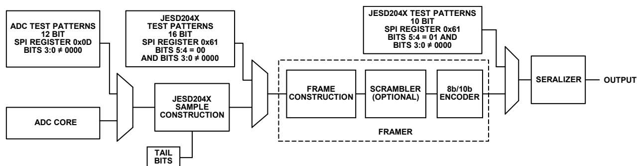
Figure 56. Test Modes
