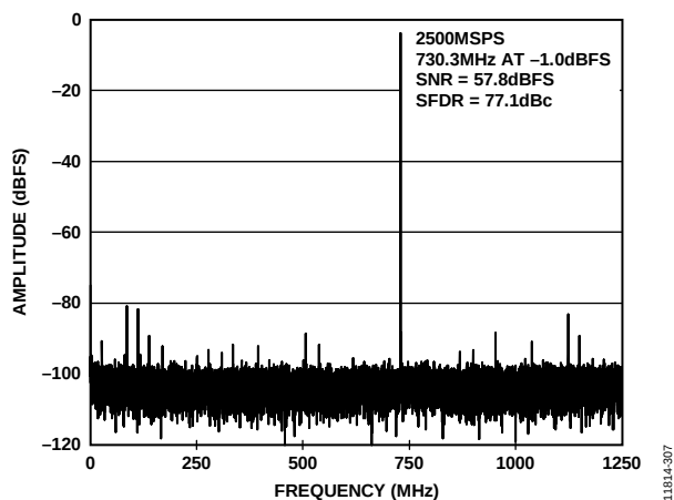
Figure 7. FFT Plot at 2.5 GSPS, f_{IN} = 730.3 MHz at AIN (SFDR = 77.8 dBc, SNR = 57.8 dBFS)
