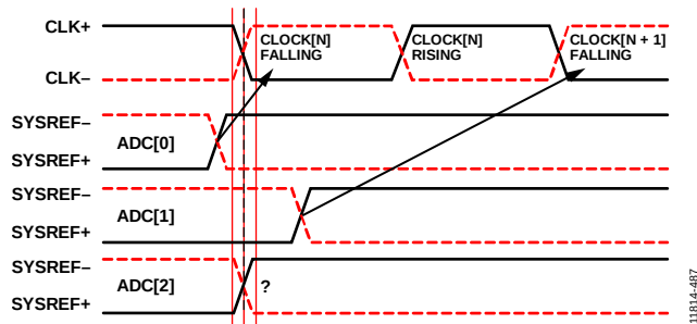
Figure 82. SYSREF± Case From Three ADCs Having Various Phase Delays Relative to the Falling Edge of the Encode Clock and will be Latched on Different Sample Clock Edges CLK±[N] or CLK±[N + 1]
