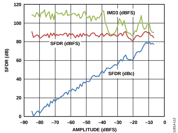
Figure 17. Two Tone SFDR and IMD3 vs. Analog Input Amplitude at 2.0 GSPS at 1800 MHz AIN
