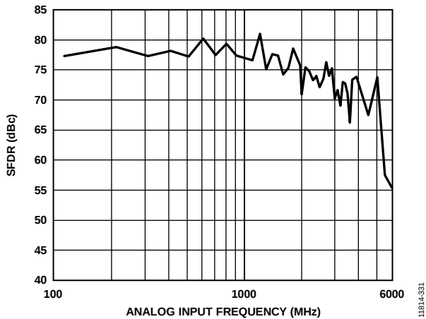
Figure 31. SFDR vs. AIN frequency at 2.5 GSPS (Input Network in Figure 60 Used &lt;2 GHz, Input Network in Figure 59 used &gt;2 GHz)
