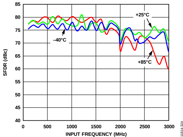
Figure 24. SFDR at 2.5 GSPS vs. Temperature (Input Network in Figure 60 Used <2 GHz, Input Network in Figure 59 Used >2 GHz)
