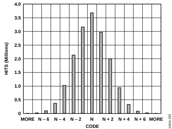
Figure 33. Input Referred Noise Histogram with 2.5 GHz Sample Clock
