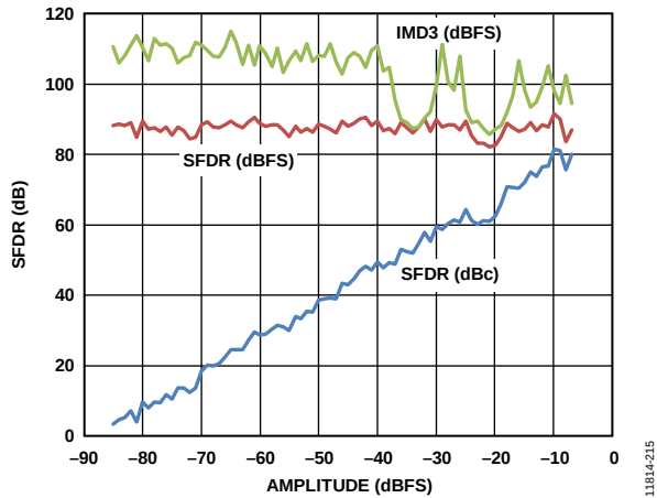
Figure 18. Two Tone SFDR and IMD3 vs. Analog Input Amplitude at 2.0 GSPS at 230 MHz AIN
