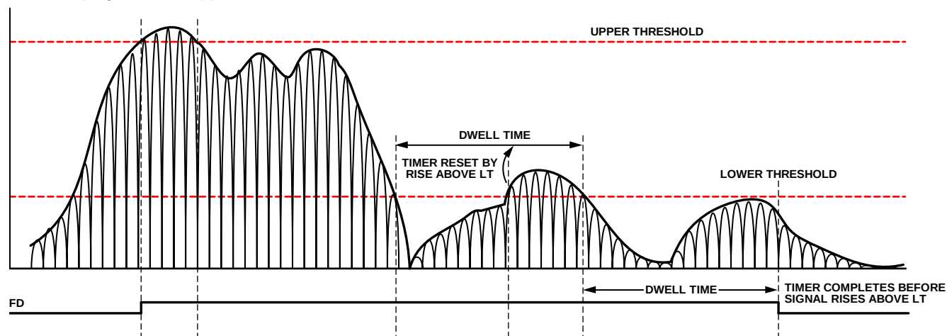
Figure 55. Fast Detection Bit
