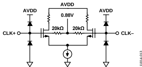
Figure 48. Equivalent Clock Input Circuit
