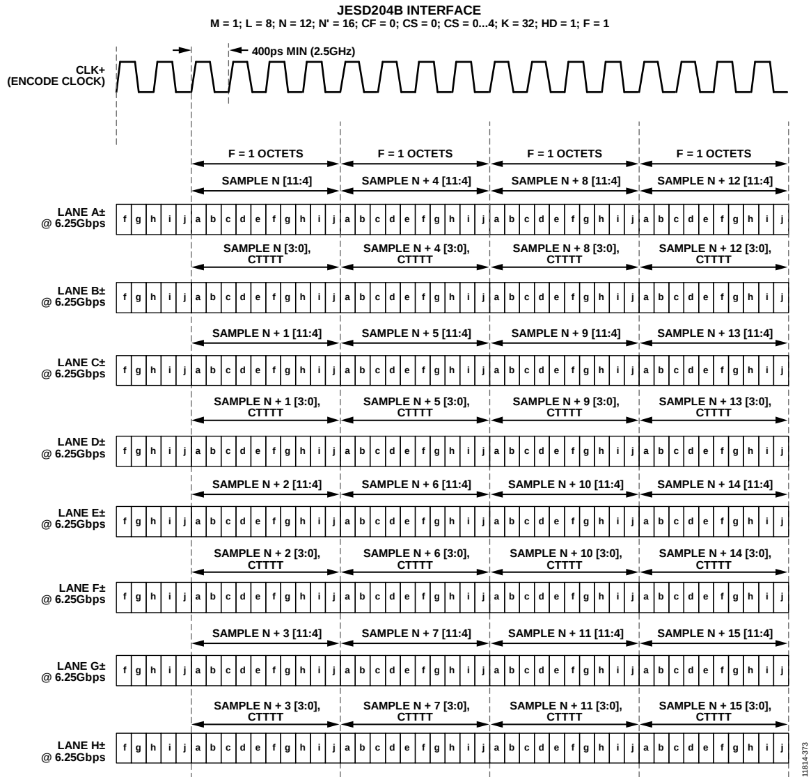
Figure 68. JESD204B Lane Data Mapping
