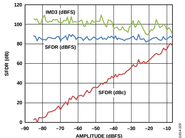
Figure 29. Two Tone SFDR and IMD3 vs. Analog Input Amplitude at 2.5 GSPS at 730 MHz AIN
