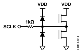
Figure 46. Equivalent SCLK Circuit
