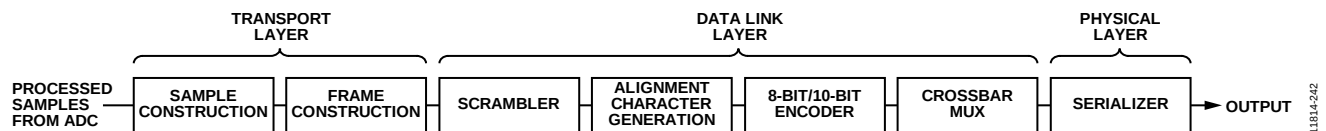
Figure 67. Data Flow
