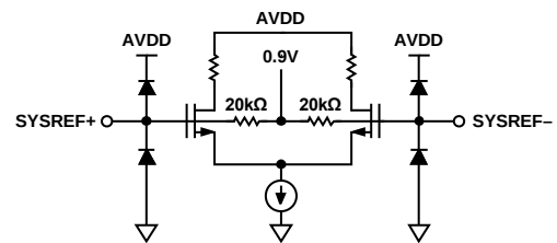
Figure 54. Equivalent SYSREF± Input Circuit
