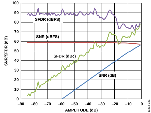
Figure 21. SNR/SFDR vs. Analog Input Amplitude at 2.5 GSPS, f_{IN} = 1811 MHz at AIN
