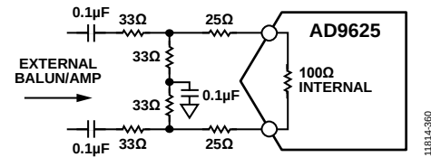
Figure 59. Input Network Example for Passive Balun and >2 GHz ADC Bandwidth
