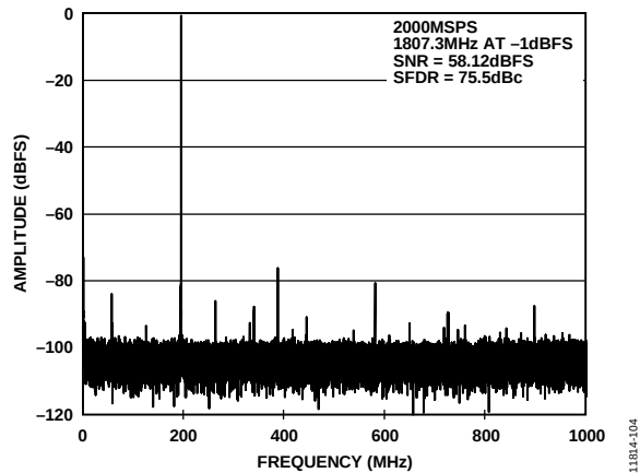
Figure 12. FFT Plot at 2.0 GSPS, f_{IN} = 1807.3 MHz at AIN (SFDR = 75.5 dBc, SNR = 58.1 dBFS)
