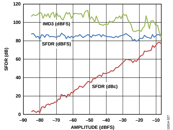
Figure 27. Two Tone SFDR and IMD3 vs. Analog Input Amplitude at 2.5 GSPS at 1800 MHz AIN
