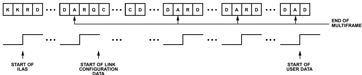
Figure 70. Initial Lane Alignment Sequence
