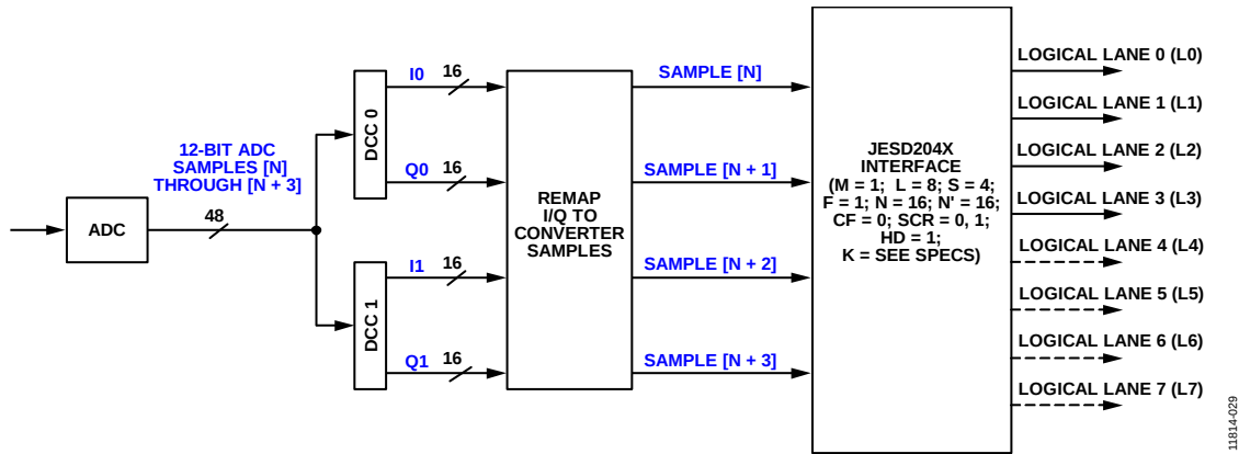
Figure 74. DDC Mapping
