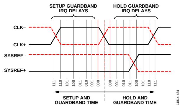
Figure 79. SYSREF± Edge Falls Within the Guardbanded Hold Time Window and Triggers an IRQ Error
