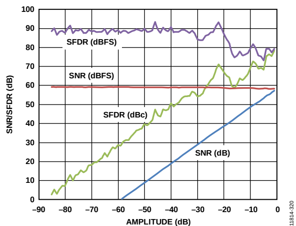
Figure 20. SNR/SFDR vs. Analog Input Amplitude at 2.5 GSPS, f_{IN} = 241 MHz at AIN
