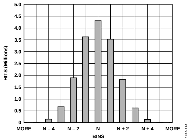
Figure 19. Input Referred Noise Histogram with 2.0 GHz Sample Clock
