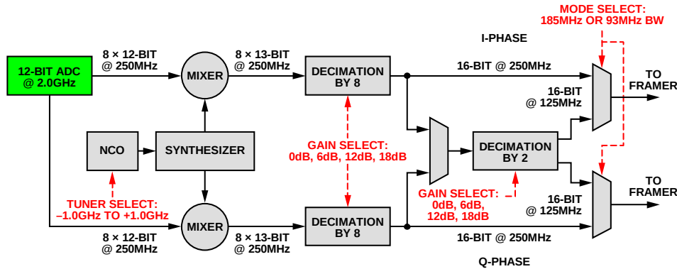
Figure 62. Digital Downconverter Block Diagram Operating at 2.0 GSPS
