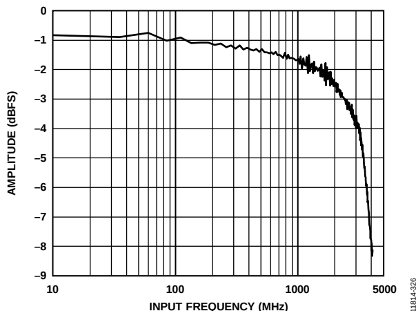
Figure 26. Full Power Input Bandwidth (Input Network in Figure 60 Used <2 GHz, Input Network in Figure 59 Used >2 GHz)
