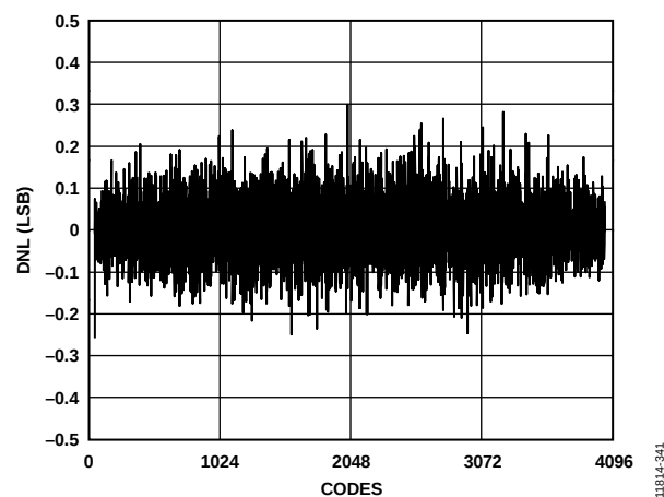
Figure 41. Differential Nonlinearity (DNL), \pm 0.3 LSB at 2.5 GSps
