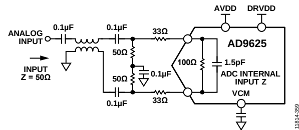
Figure 58. Input Network Example for Passive Balun with High Bandwidth
