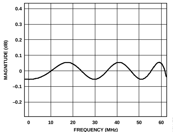
Figure 66. Magnitude Ripple in the Low Bandwidth Pass Band
