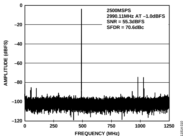
Figure 10. FFT Plot at 2.5 GSPS, f_{IN} = 2990.1 MHz at AIN (SFDR = 70.6 dBc, SNR = 55.3 dBFS) (Input Network in Figure 59 Used)
