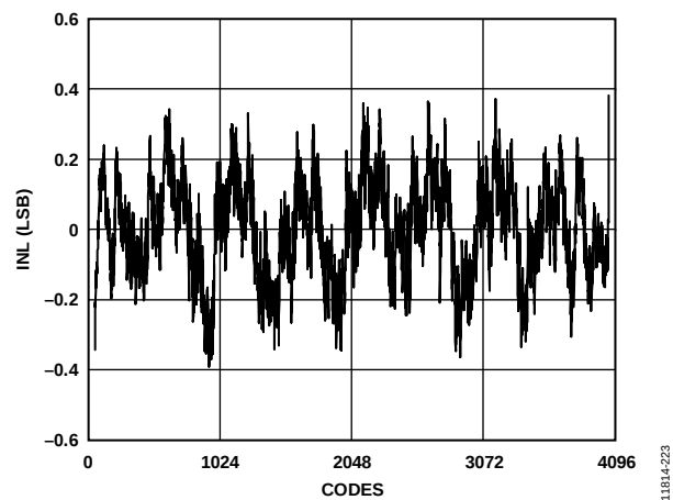
Figure 42. Integral Nonlinearity (INL), ±0.4 LSB at 2.0 GSPS
