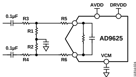
Figure 57. Recommended Front-End Network
