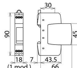
Dimension drawing DR M 2P 255
