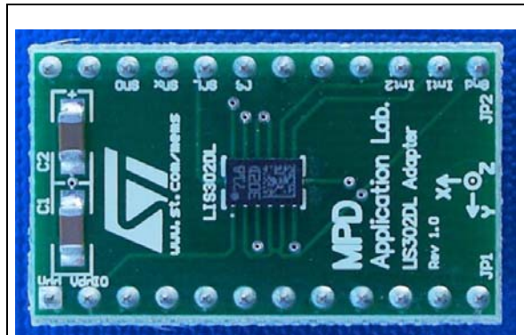
STEVAL-MKI013V1
