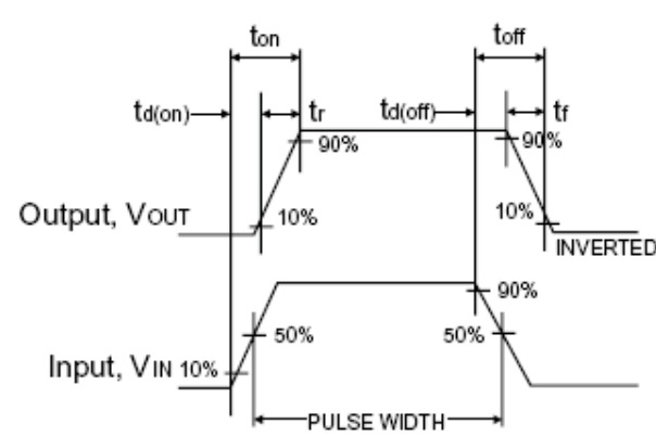
Switchin Waveforms
