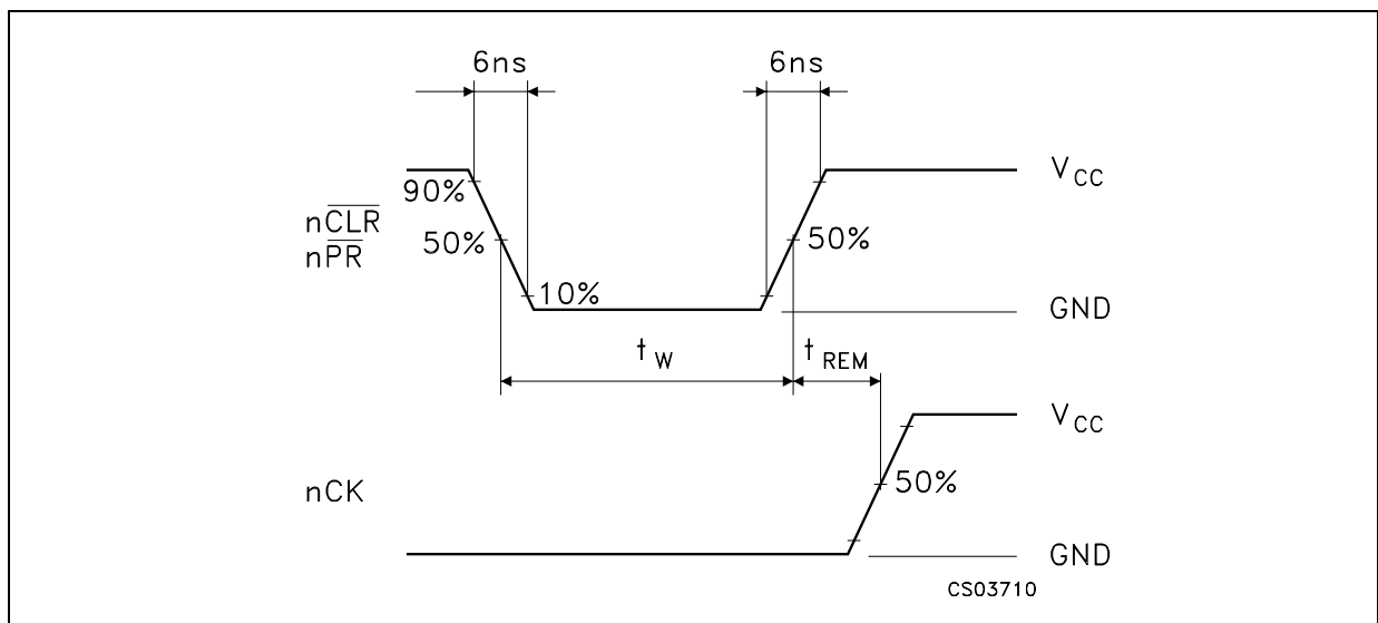
WAVEFORM 3 : MINIMUM PULSE WIDTH ( n\overline{CLR} and n\overline{PR} ), MINIMUM REMOVAL TIME ( n\overline{CLR} and n\overline{PR} TO nCK ) ( f=1\text{MHz} ; 50% duty cycle)
