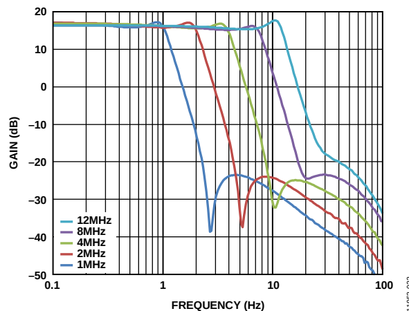
Figure 14. Filter Response
