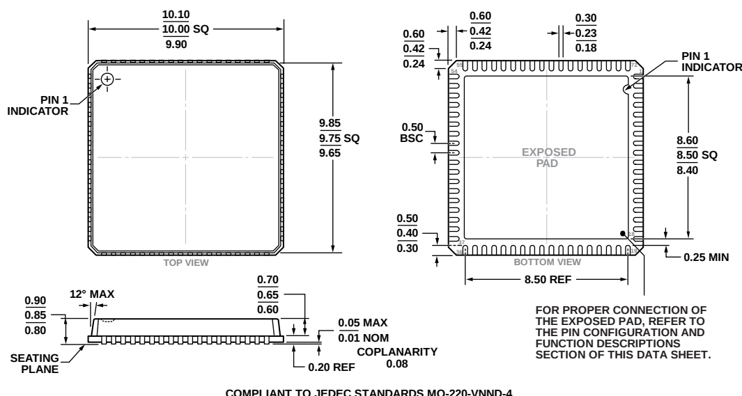
Figure 35. 72-Lead Lead Frame Chip Scale Package [LFCSP_VQ] 10 mm × 10 mm Body, Very Thin Quad (CP-72-5) Dimensions shown in millimeters
