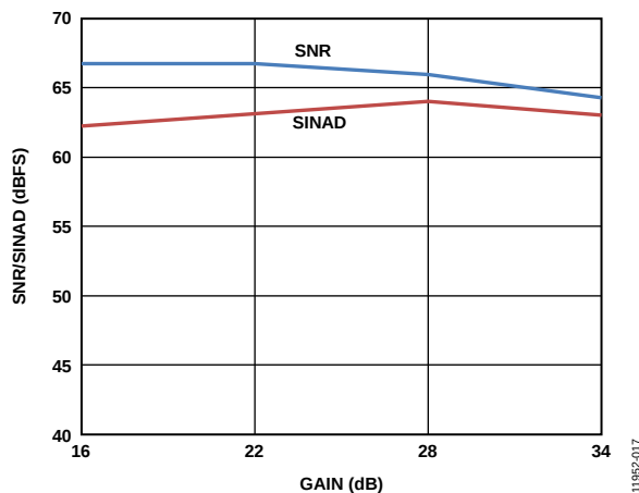
Figure 13. SNR/SINAD vs. Gain
