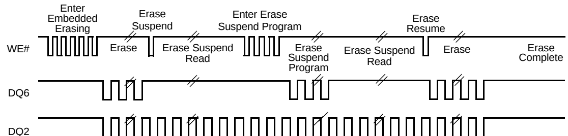
Figure 17.10 DQ2 vs. DQ6 for Erase and Erase Suspend Operations
