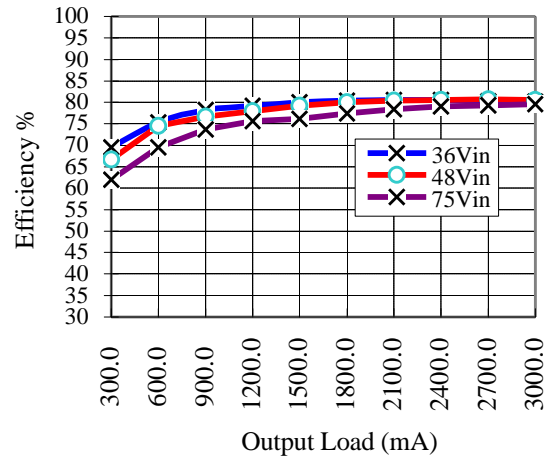
Efficiency vs. Load @ +25° Ambient, ASA03F48-L
