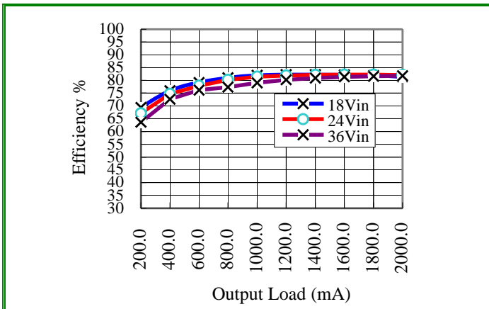
Efficiency vs. Load @ +25° Ambient, ASA02A24-L
