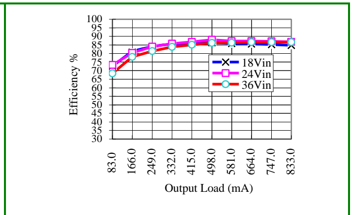
Efficiency vs. Load @ +25° Ambient, ASA00B24-L
