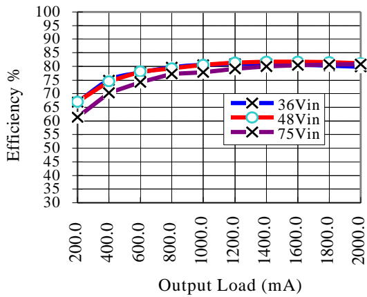
Efficiency vs. Load @ +25° Ambient, ASA02A48-L
