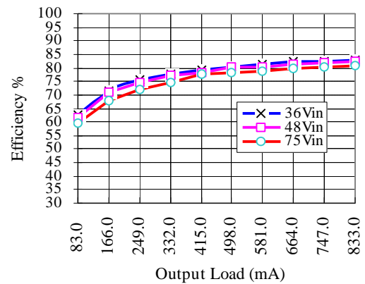
Efficiency vs. Load @ +25° Ambient, ASA00B48-L
