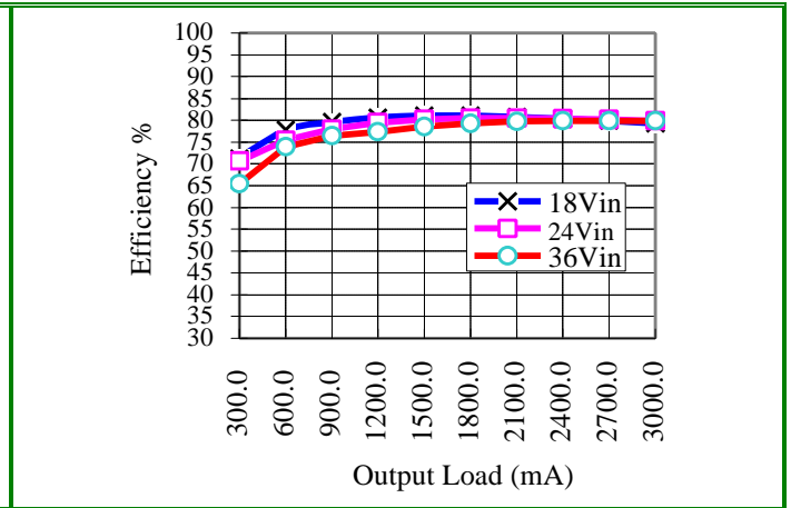
Efficiency vs. Load @ +25° Ambient, ASA03F24-L
