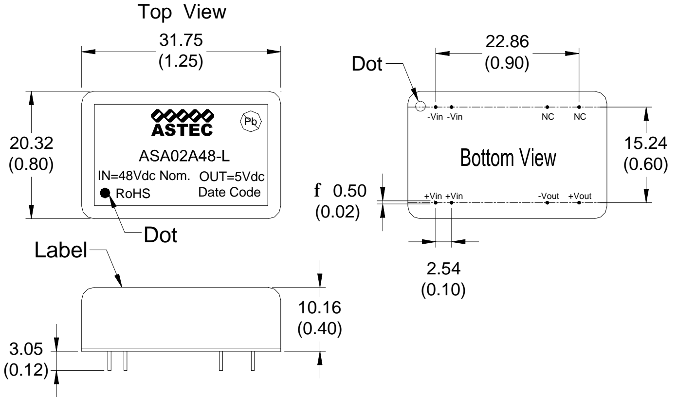
Outline Drawing for ASA Series
