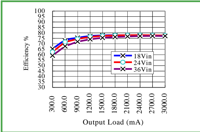
Efficiency vs. Load @ +25° Ambient, ASA03G24-L
