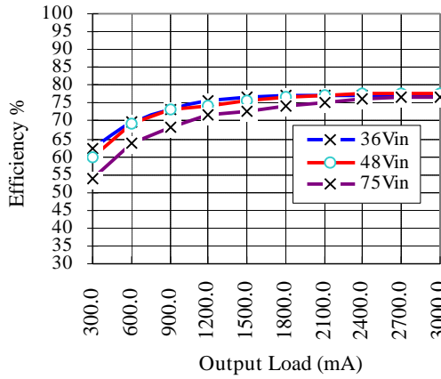
Efficiency vs. Load @ +25° Ambient, ASA03G48-L
