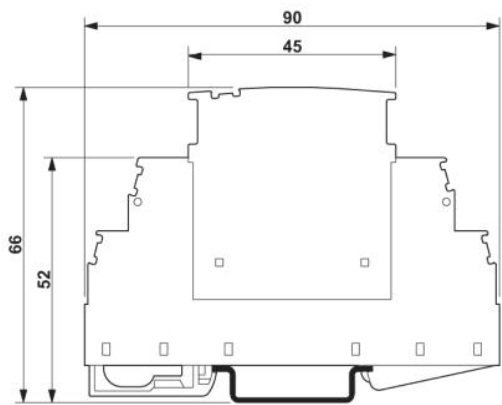
Dimensioned drawing
