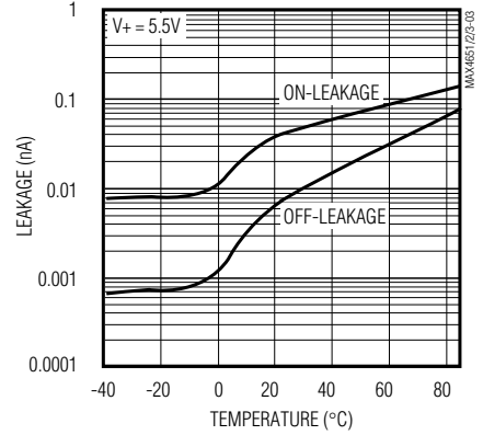
ON/OFF-LEAKAGE CURRENT vs. TEMPERATURE
