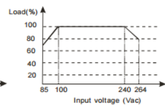
Input voltage vs load
