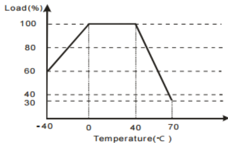
Temperature vs load
