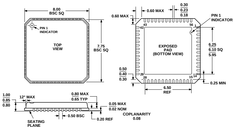
Figure 82. 56-Lead Lead Frame Chip Scale Package [LFCSP] 8 mm × 8 mm Body, Very Thin Quad (CP-56) Dimensions shown in millimeters
