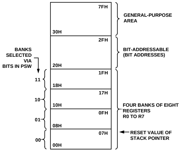
Figure 8. Lower 128 Bytes of Internal Data Memory
