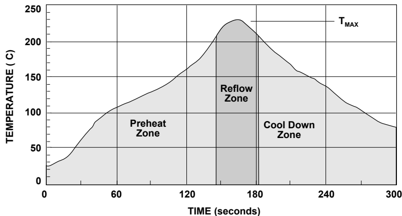
Figure 14. Surface Mount Assembly Profile.
