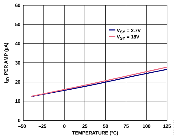
Figure 26. Supply Current per Amplifier vs. Temperature
