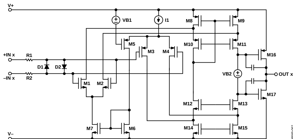
Figure 61. Simplified Schematic
