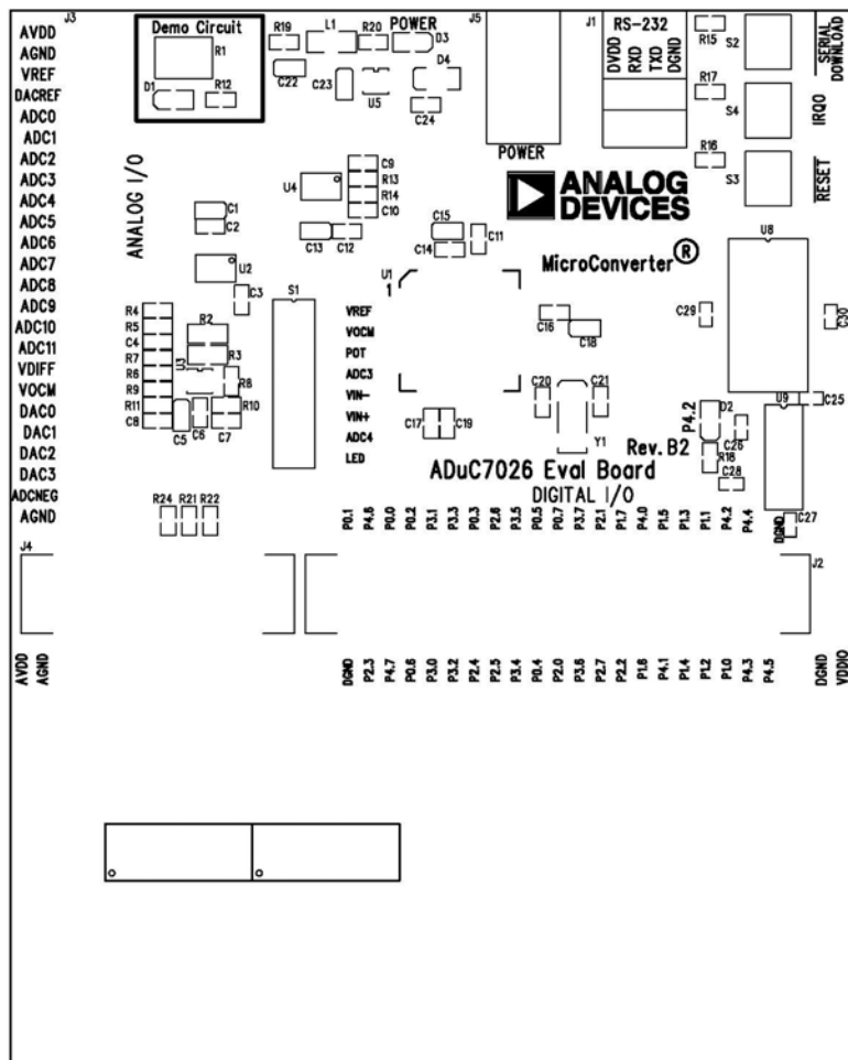
Figure 6. Evaluation Board Silkscreen
