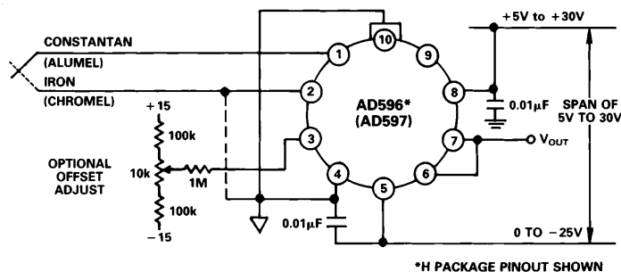
Figure 1. Temperature Proportional Output Connection
