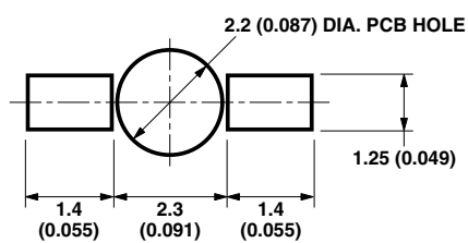
Figure 8. Recommended soldering pattern for HSMx-C265.
