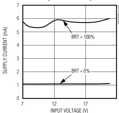
SUPPLY CURRENT vs. INPUT VOLTAGE (DPWM DIMMING)
