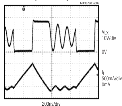
SWITCHING WAVEFORMS (BRT = 100%)
