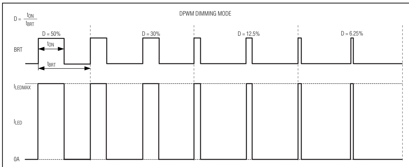
Figure 5. LED Current Control Using DPWM Dimming Mode
