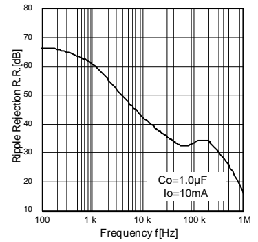
Fig. 17 Ripple Rejection (BH33RB1WGUT)
