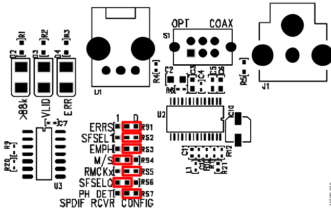
Figure 16. S/PDIF Mode Selection Resistors
