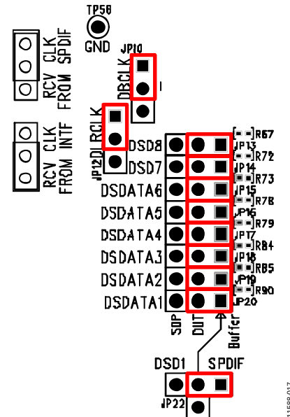
Figure 17. S/PDIF Data and Clock Routing
