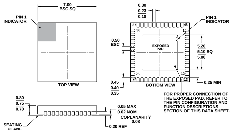
Figure 40. 48-Lead Lead Frame Chip Scale Package [LFCSP_WQ] 7 mm × 7 mm Body, Very Very Thin Quad CP-48-4
