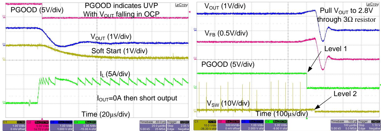
Figure 24. Over-Current Protection with Heavy Load Applied
