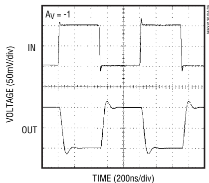
MAX4131 SMALL-SIGNAL TRANSIENT RESPONSE (INVERTING)
