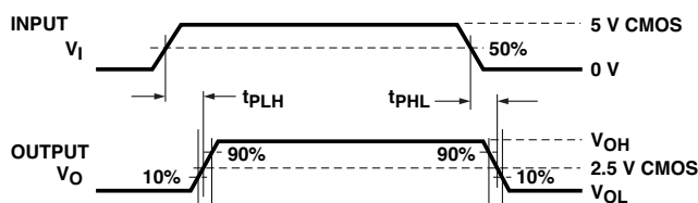
Figure 9. Timing diagram to illustrate propagation delay, t_{plh} and t_{phl} .
