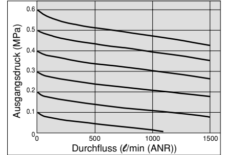
AC40-06 Rc 3/4
