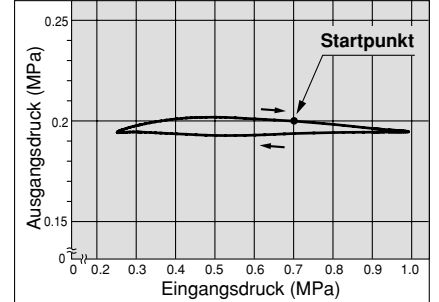
AC40-06
