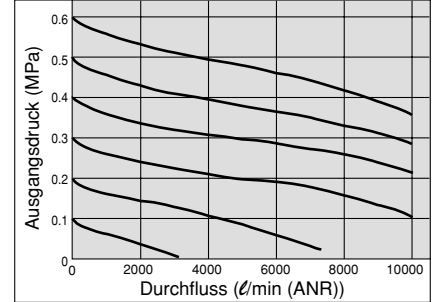
AC60 Rc 1
