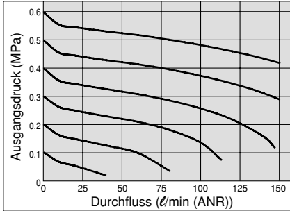
AC30 Rc 3/8
