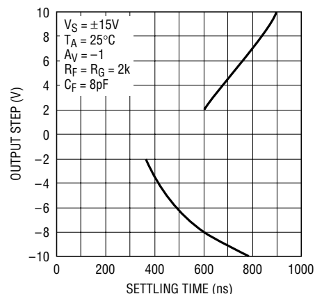
Settling Time to 150μV vs Output Step
