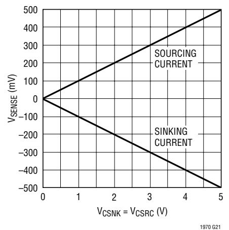
Full Range Current Sense Transfer Curve
