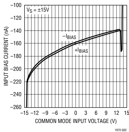
Input Bias Current vs V_{\text{CM}}
