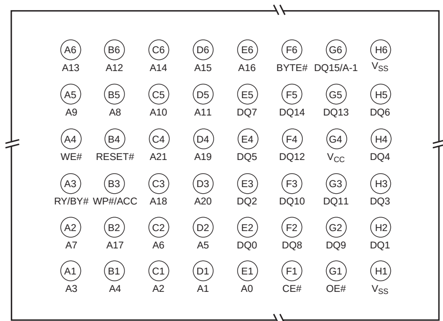
Figure 4.2 48-ball FBGA
