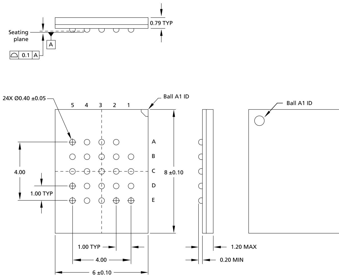
Figure 48: T-PBGA-24b05/6mm x 8mm
