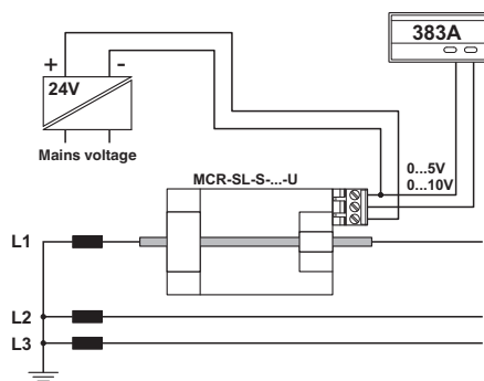
Current measurement
