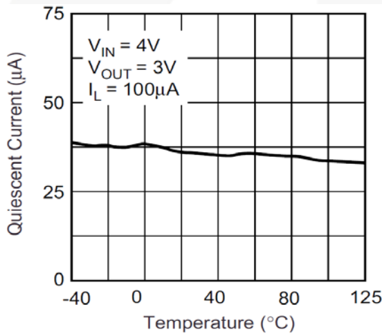
Figure 17. Ground Pin Current
