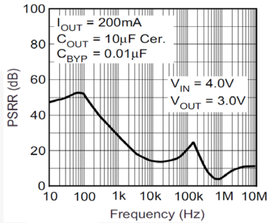
Figure 10. Power Supply Rejection Ratio
