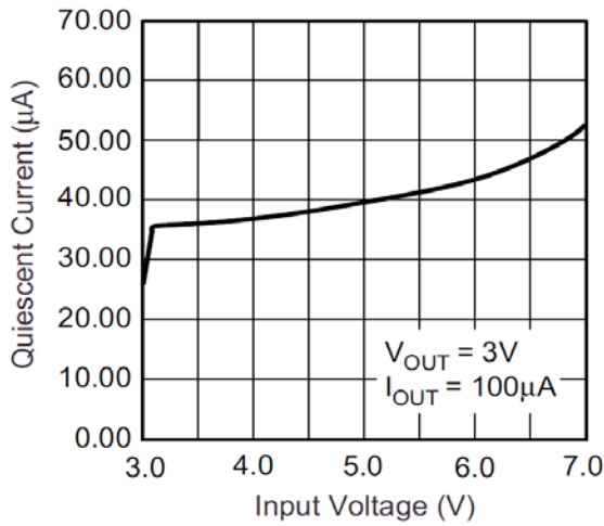
Figure 15. Ground Pin Current
