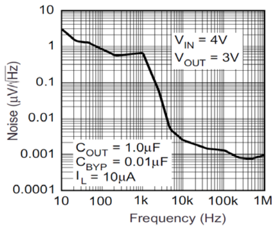
Figure 13. Noise Performance
