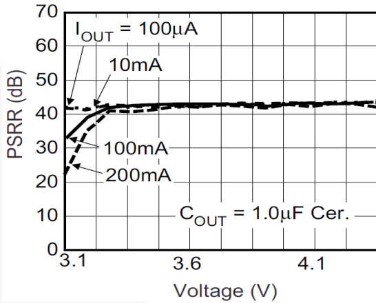
Figure 11. PSRR vs. Voltage Drop
