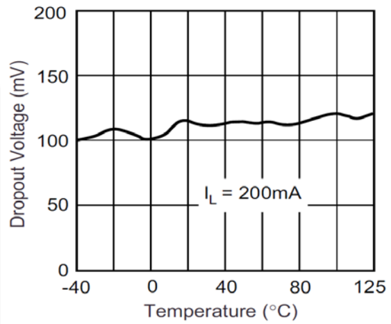
Figure 22. Dropout Voltage
