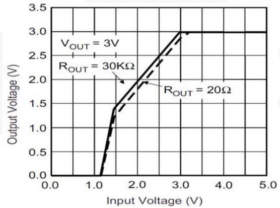
Figure 20. Dropout Characteristics
