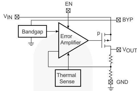
Figure 1. Block Diagram
