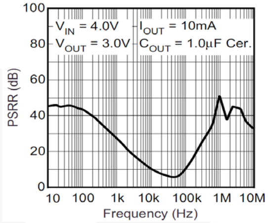
Figure 4. Power Supply Rejection Ratio
