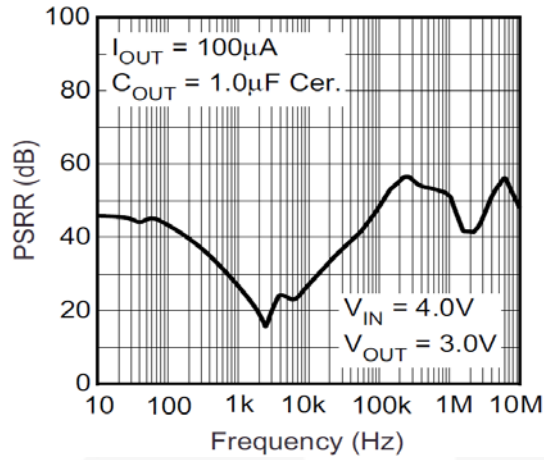
Figure 3. Power Supply Rejection Ratio
