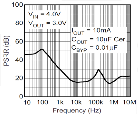
Figure 8. Power Supply Rejection Ratio
