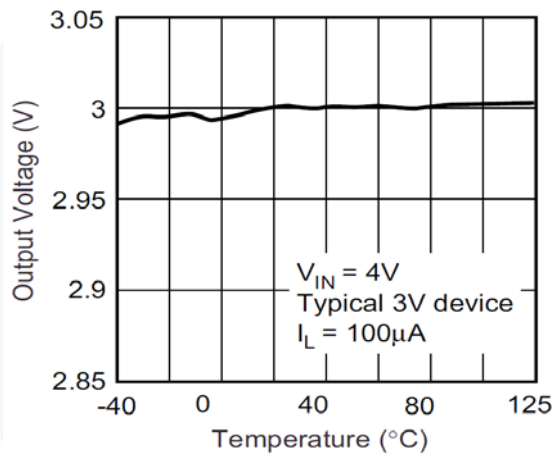
Figure 23. Out Voltage vs. Temperature
