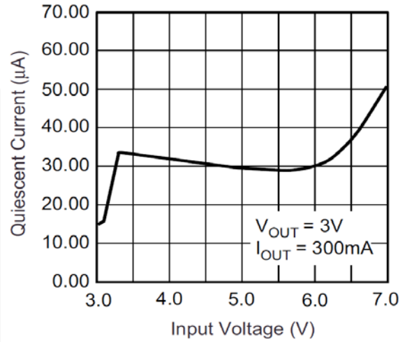
Figure 16. Ground Pin Current
