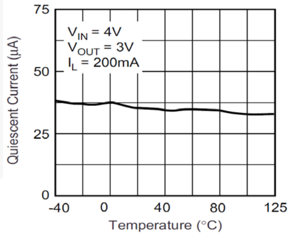
Figure 18. Ground Pin Current
