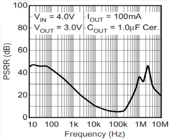
Figure 5. Power Supply Rejection Ratio
