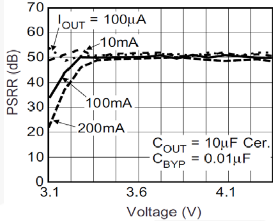
Figure 12. PSRR vs. Voltage Drop
