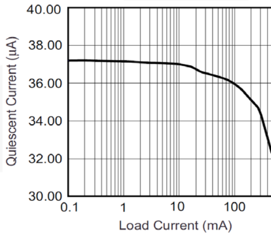
Figure 14. Ground Pin Current
