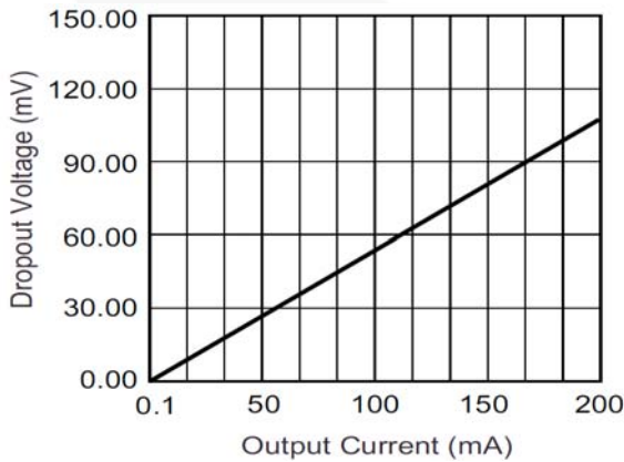
Figure 19. Dropout Voltage
