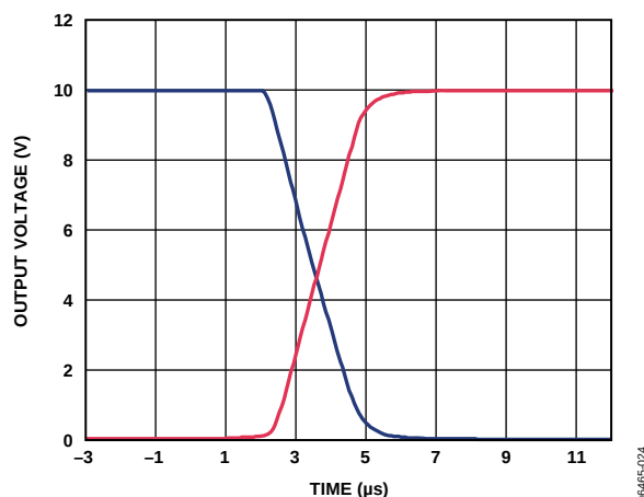
Figure 27. Full-Scale Settling, +10 V Range
