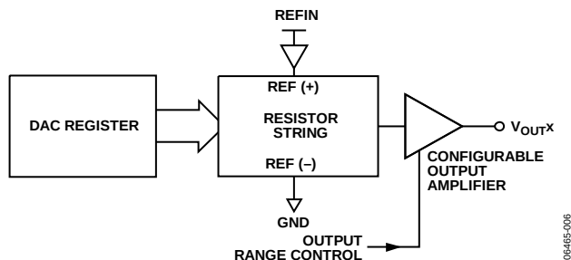
Figure 44. DAC Architecture Block Diagram
