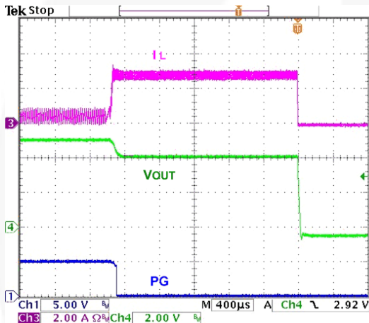
Figure 19. Overload Protection
