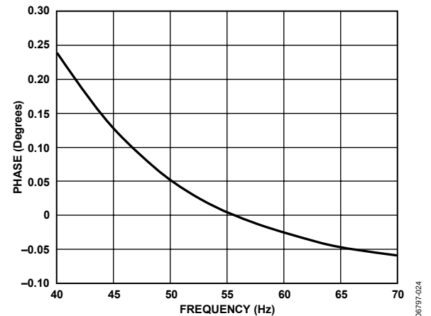
Figure 26. Phase Error Between Channels (40 Hz to 70 Hz)
