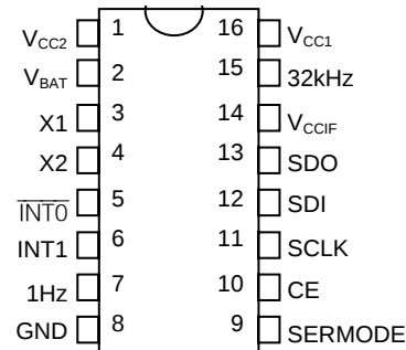
DIP (300 mils)
